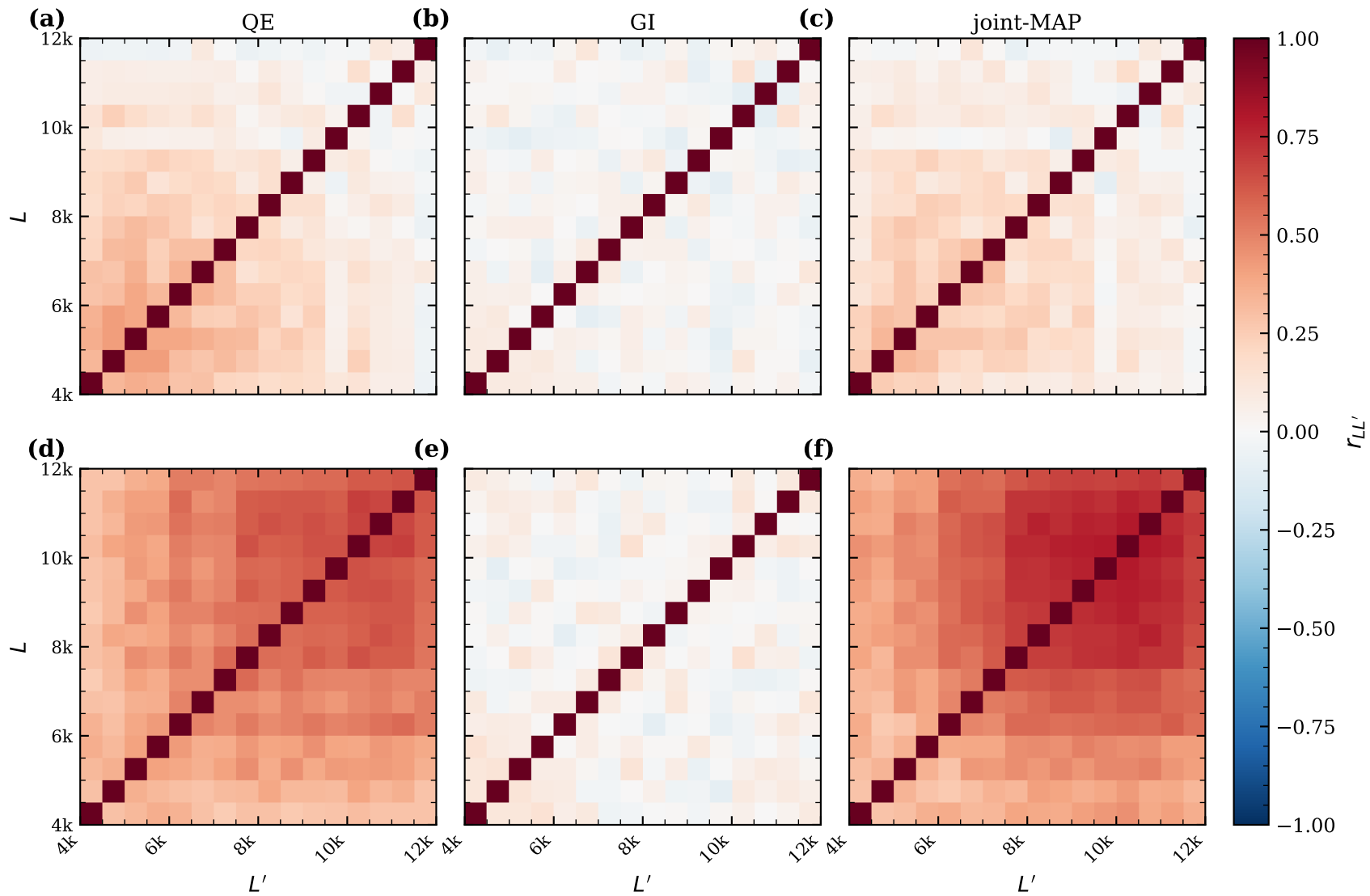
CMB-S4-like
