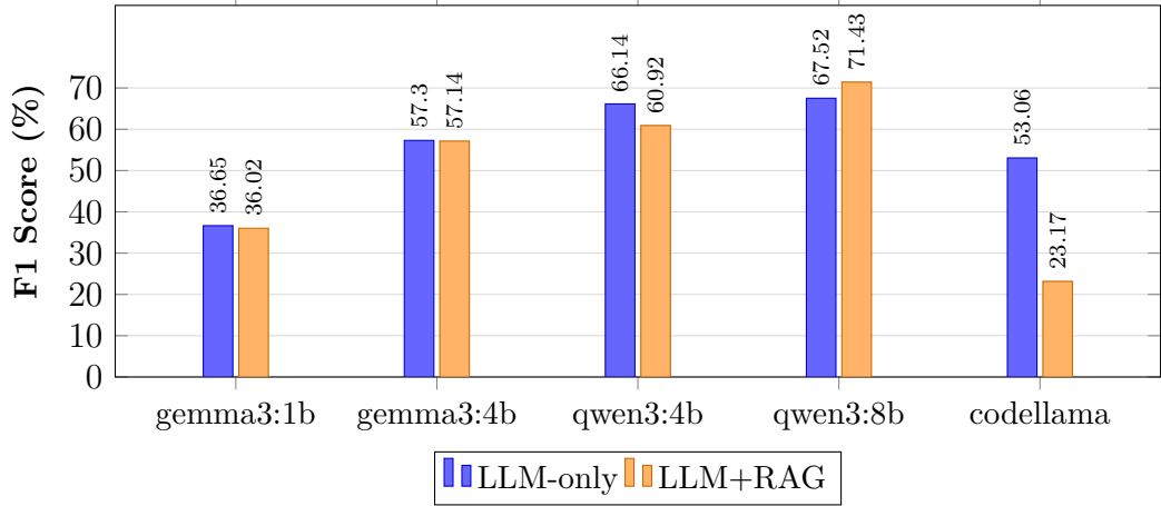
Figure 5.2.: RAG ablation: F1 comparison by model (canonical-taxonomy matching). RAG lifts qwen3:8b (+3.91), is roughly neutral on gemma3 models, slightly degrades qwen3:4b (−5.22), and severely degrades codellama (−29.89).
