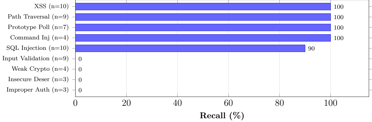
Figure 5.3.: Per-category recall for qwen3:8b+RAG , showing categories with n \geq 3 test cases. The results reveal a bimodal pattern: injection-style categories achieve 90–100% recall, while categories requiring semantic reasoning (validation, authentication, cryptography) achieve 0%.
