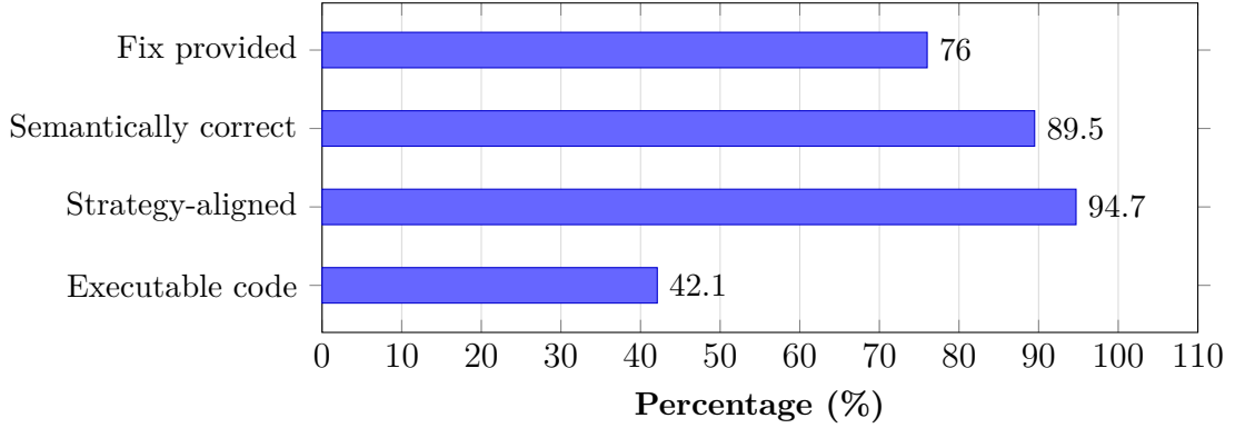
Figure 5.1.: Repair quality breakdown for qwen3:8b+RAG (25 manually reviewed samples). Most repairs are semantically correct and strategy-aligned, but less than half contain directly executable code.
