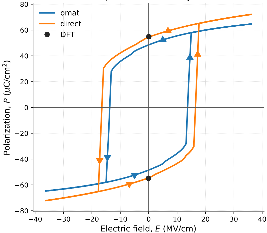
BaTiO 3 polarization-field hysteresis
