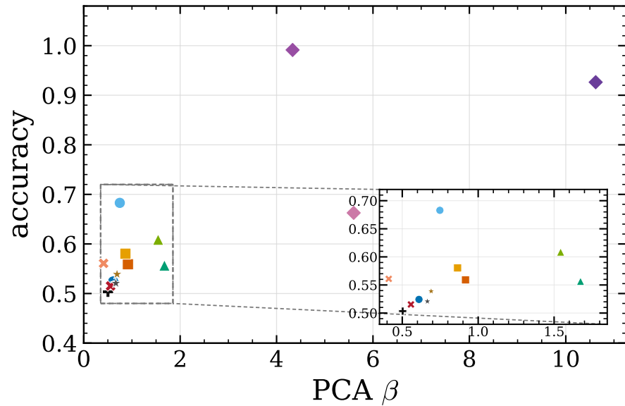
2-shot: \rho_s = 0.74
