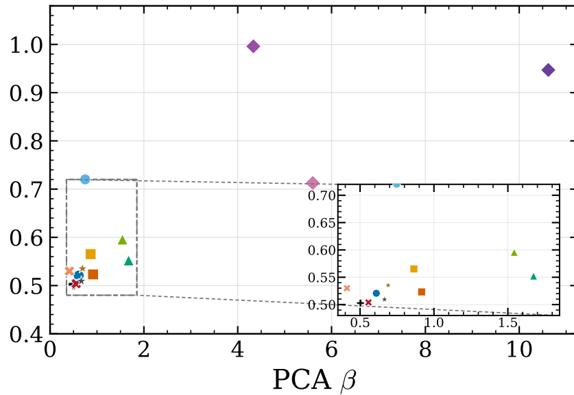
3-shot: \rho_s = 0.80
