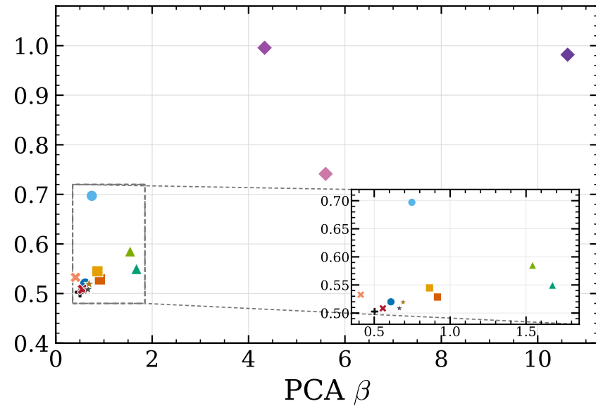
4-shot: \rho_s = 0.82
