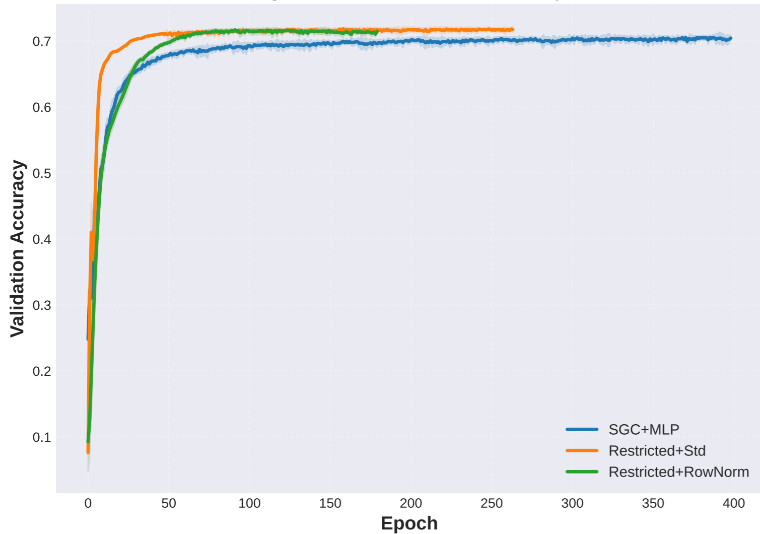
Ogbn-Arxiv: Validation Accuracy
