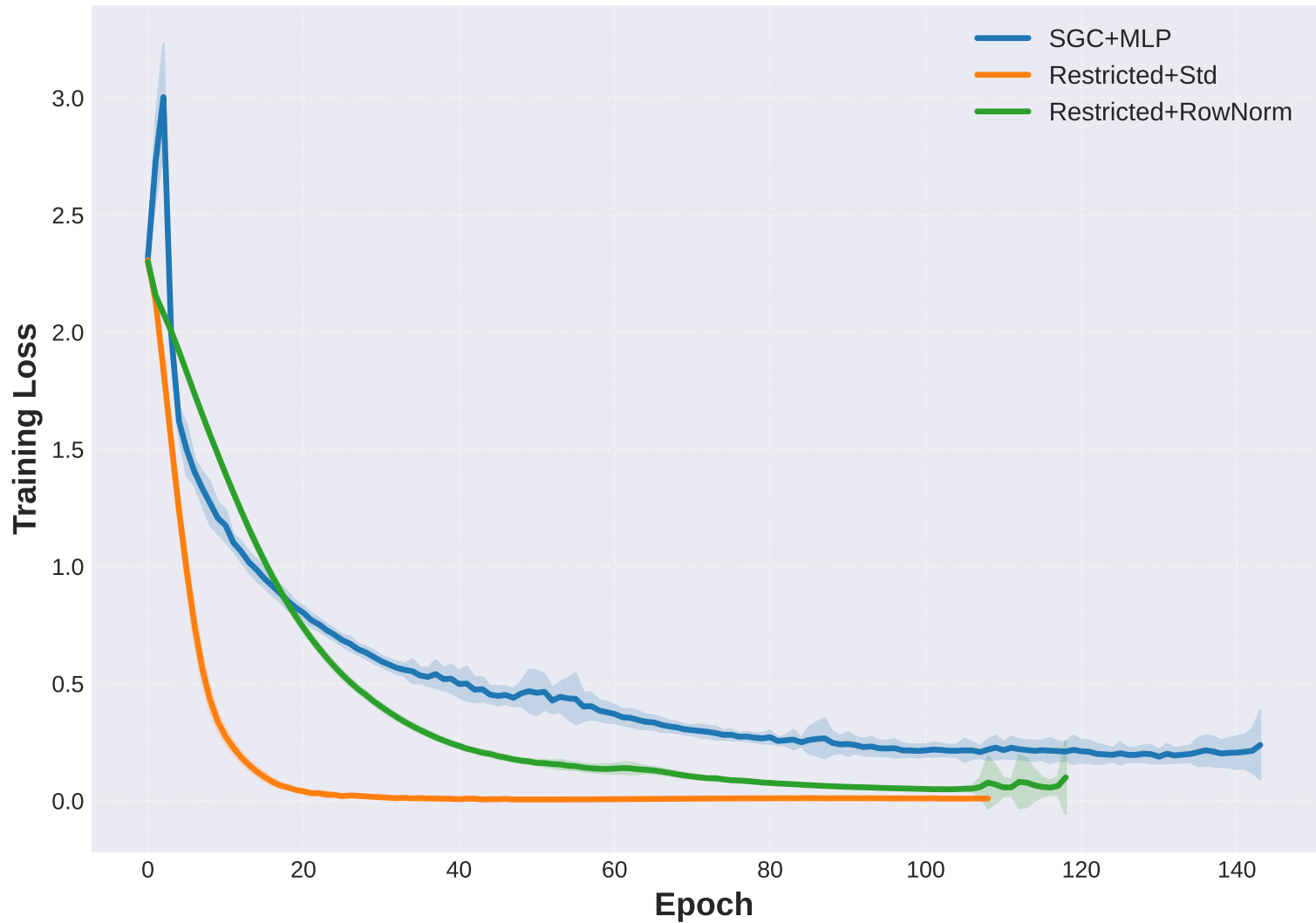
Wikics: Training Loss
