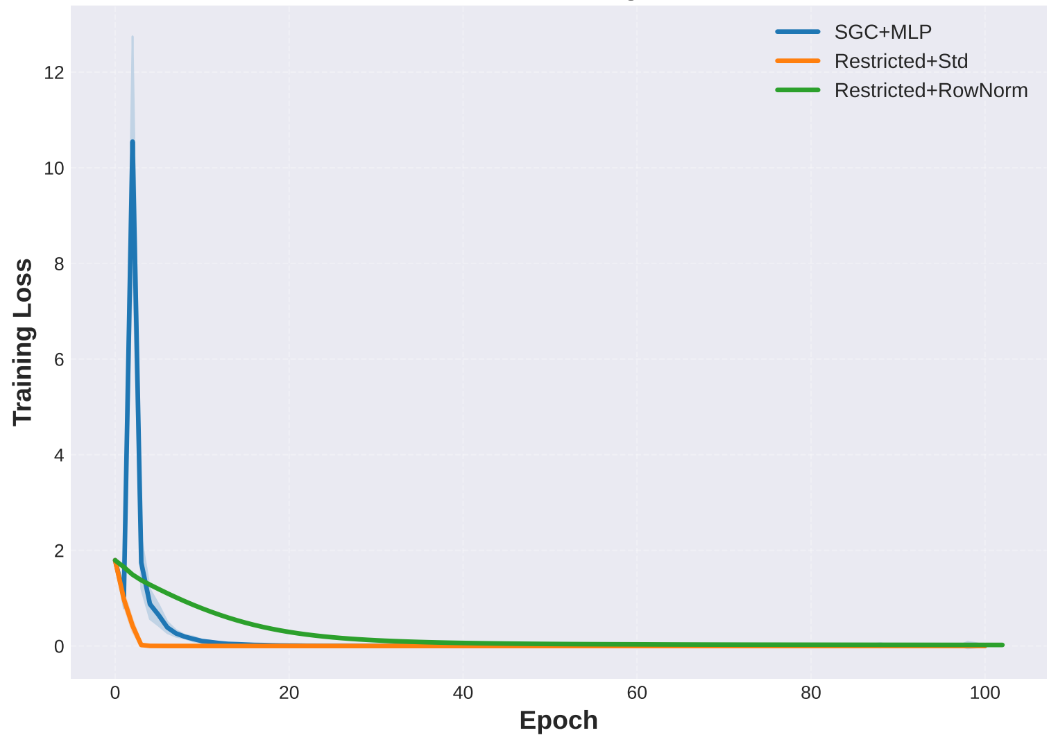
Citeseer: Training Loss
