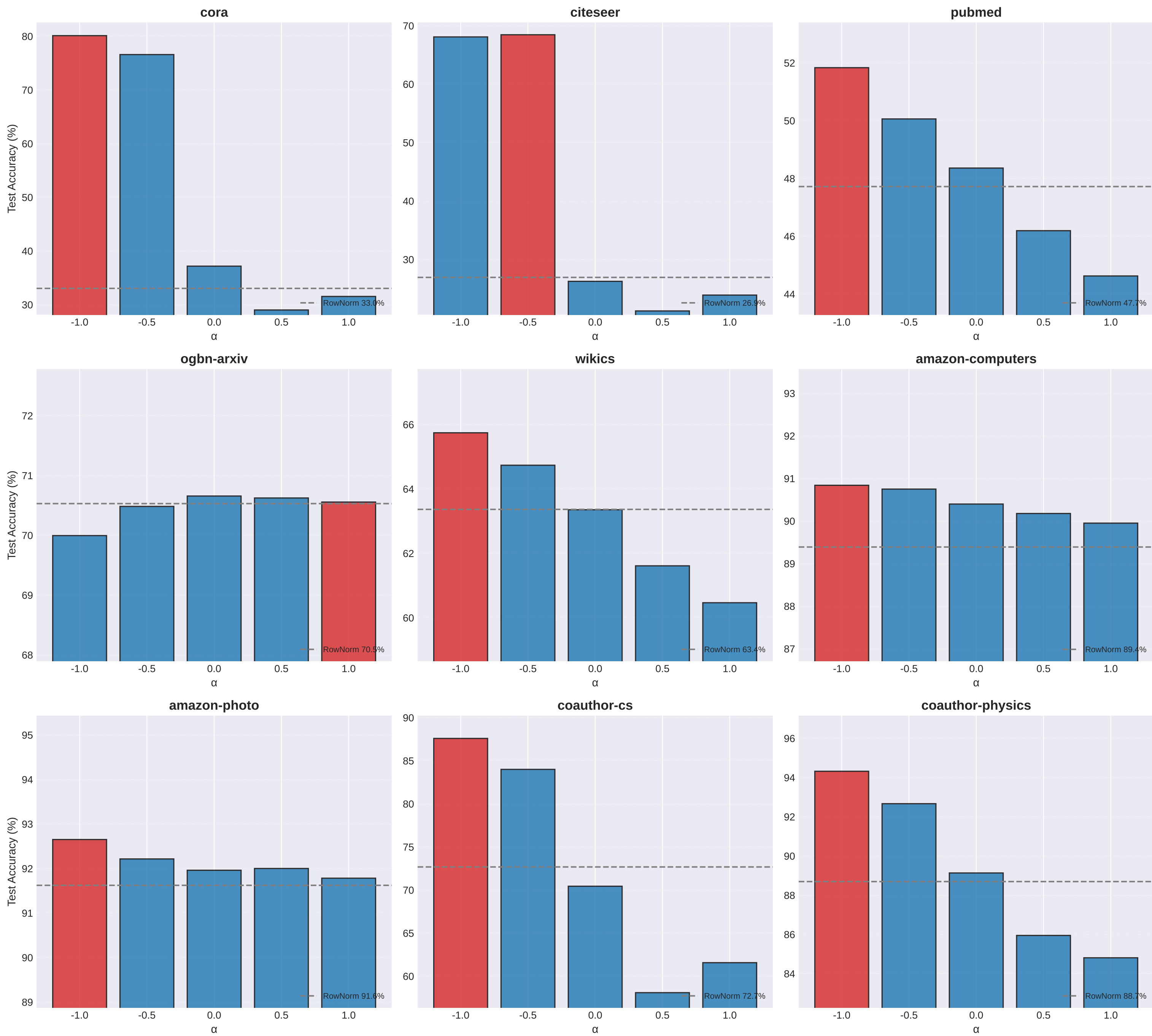
Spectral \alpha Sweep: SpectralRowNormMLP at k = 10 (red = best \alpha on val set; dashed = RowNorm baseline)
