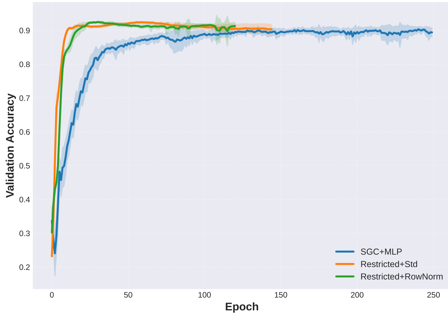
Amazon-Photo: Validation Accuracy
