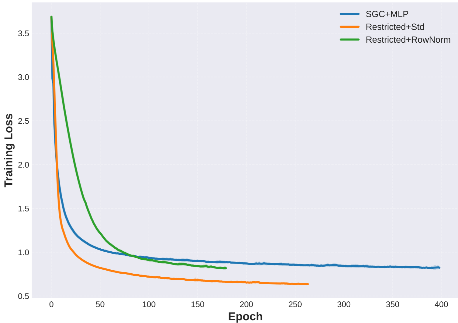
Ogbn-Arxiv: Training Loss
