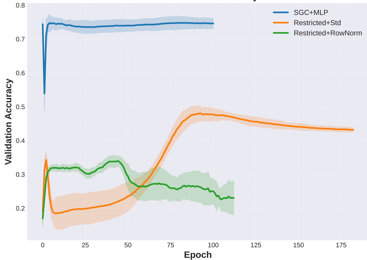
Cora: Validation Accuracy
