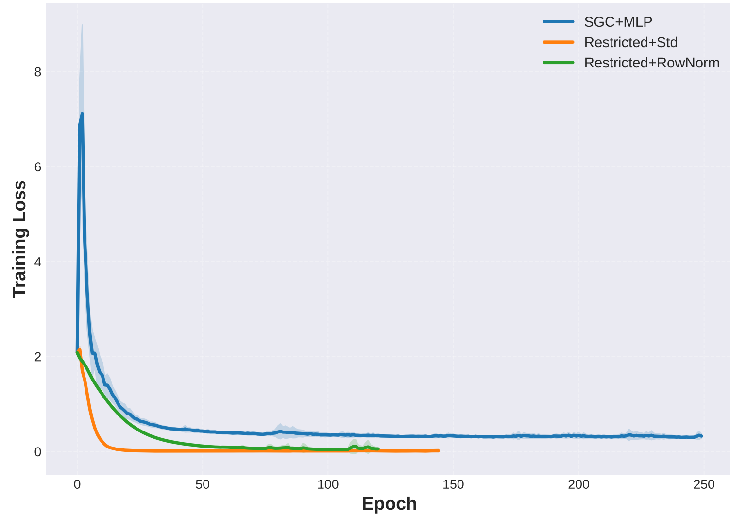
Amazon-Photo: Training Loss
