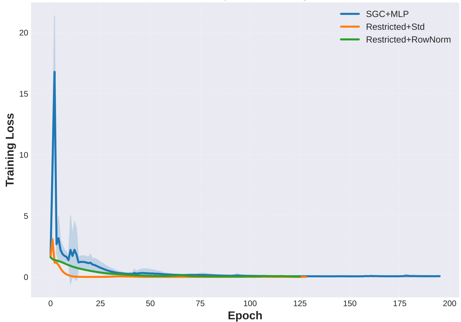
Coauthor-Physics: Training Loss
