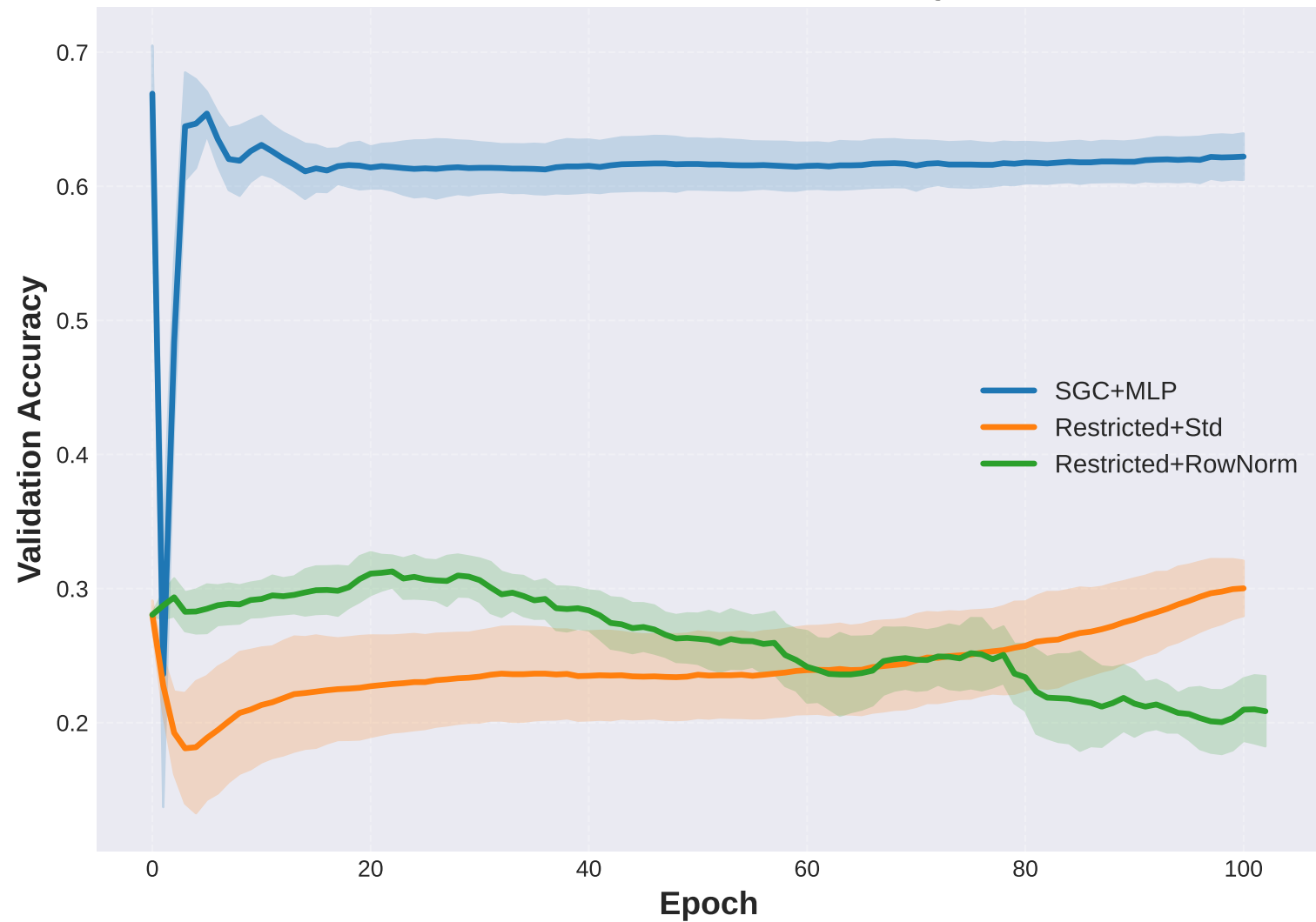
Citeseer: Validation Accuracy
