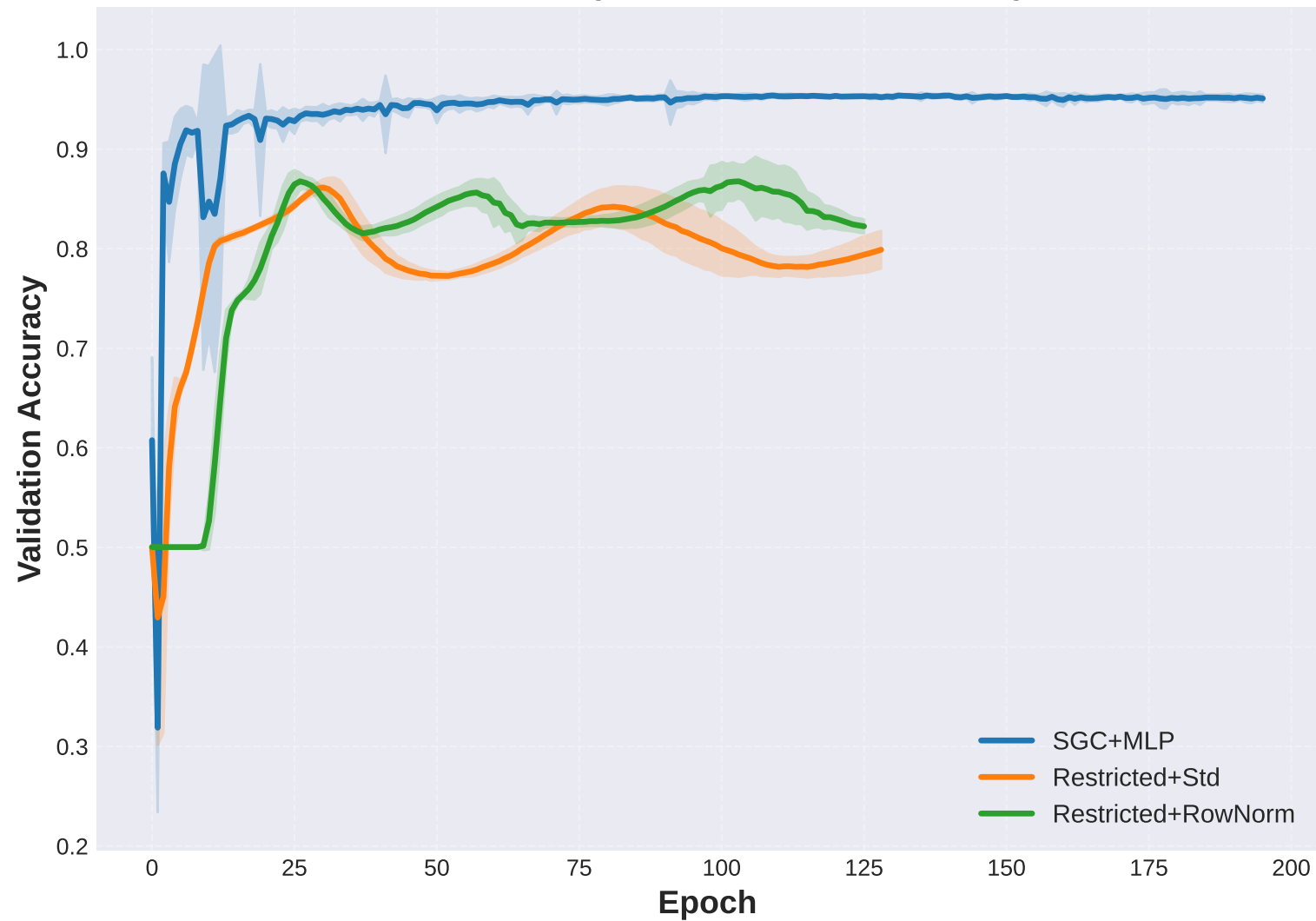
Coauthor-Physics: Validation Accuracy
