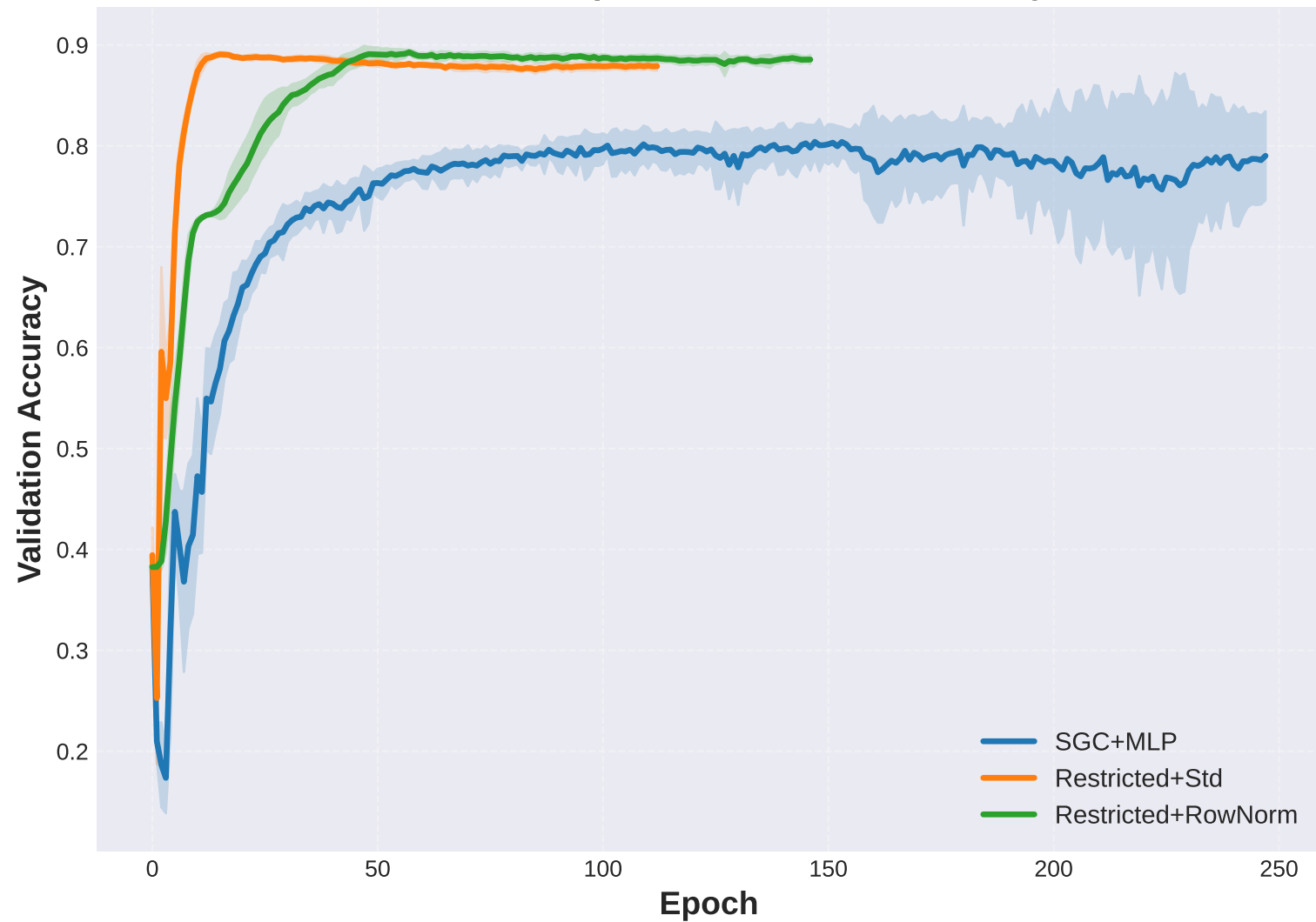
Amazon-Computers: Validation Accuracy
