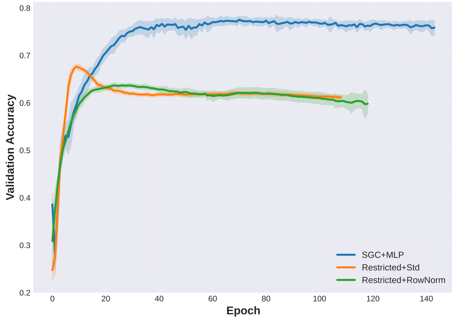
Wikics: Validation Accuracy
