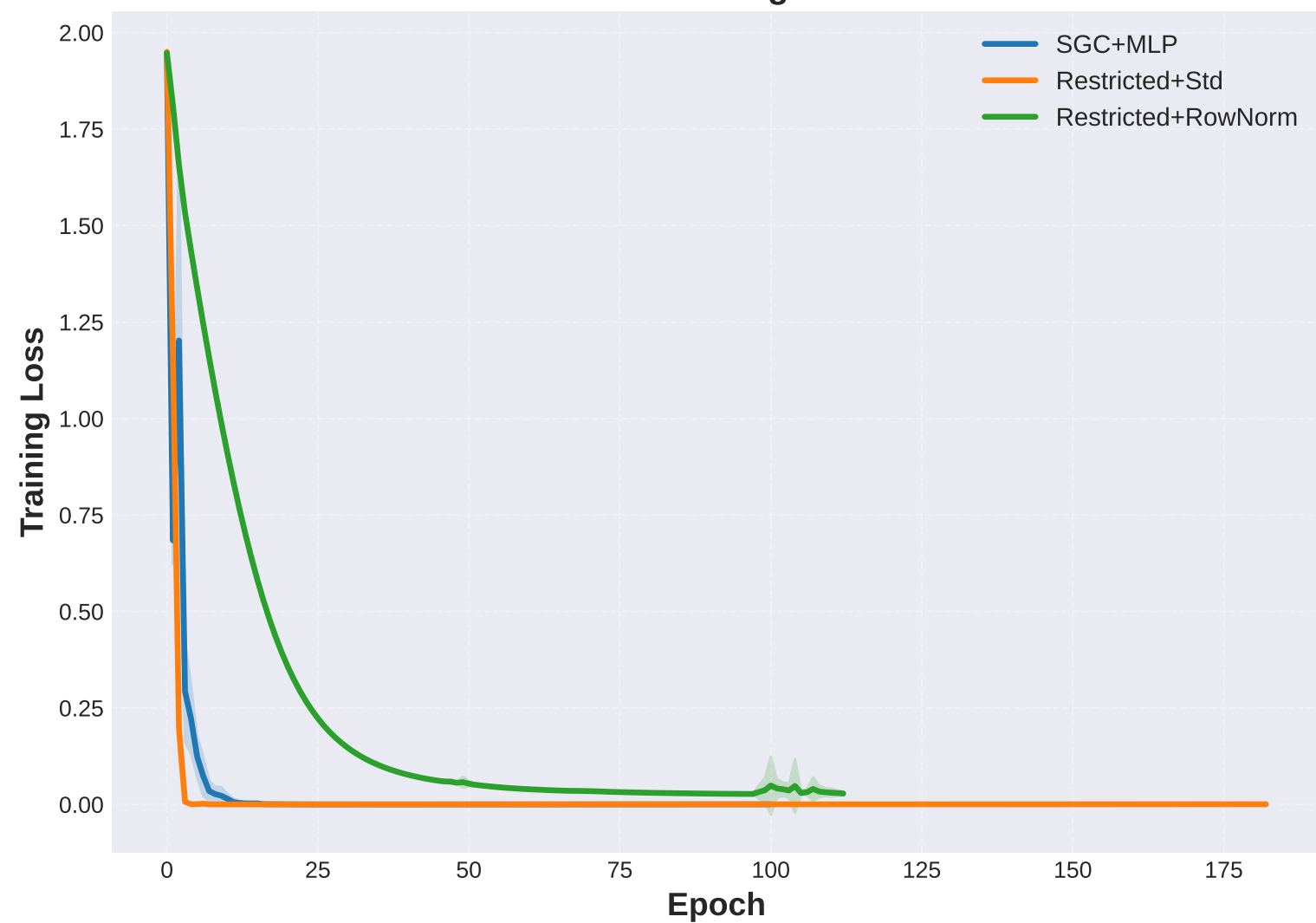
Cora: Training Loss
