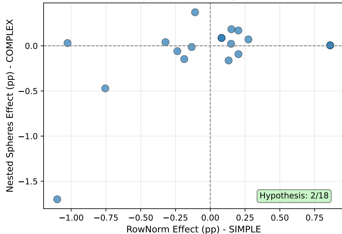
RowNorm vs Nested Spheres Hypothesis: x > 0, y < 0
