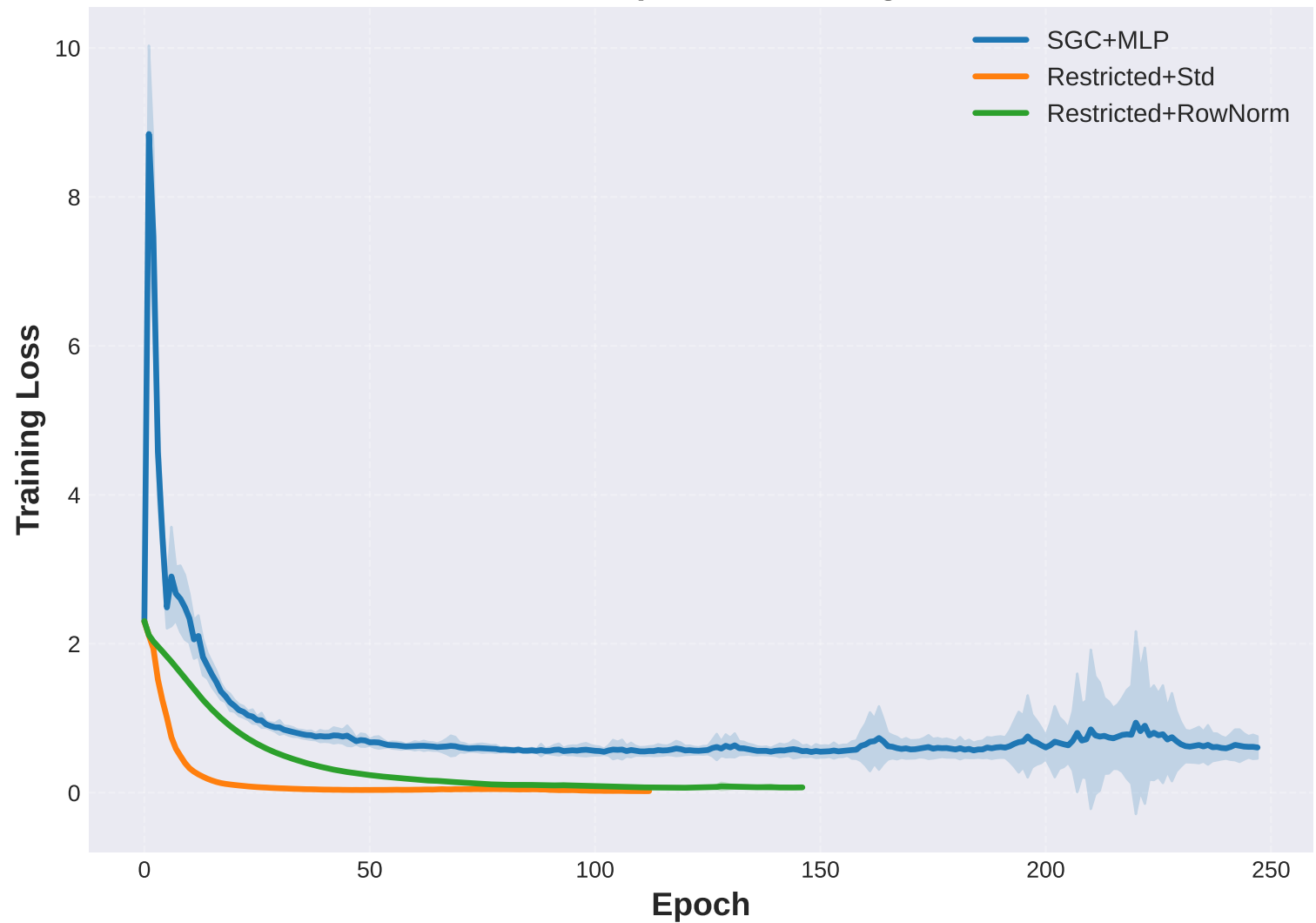
Amazon-Computers: Training Loss
