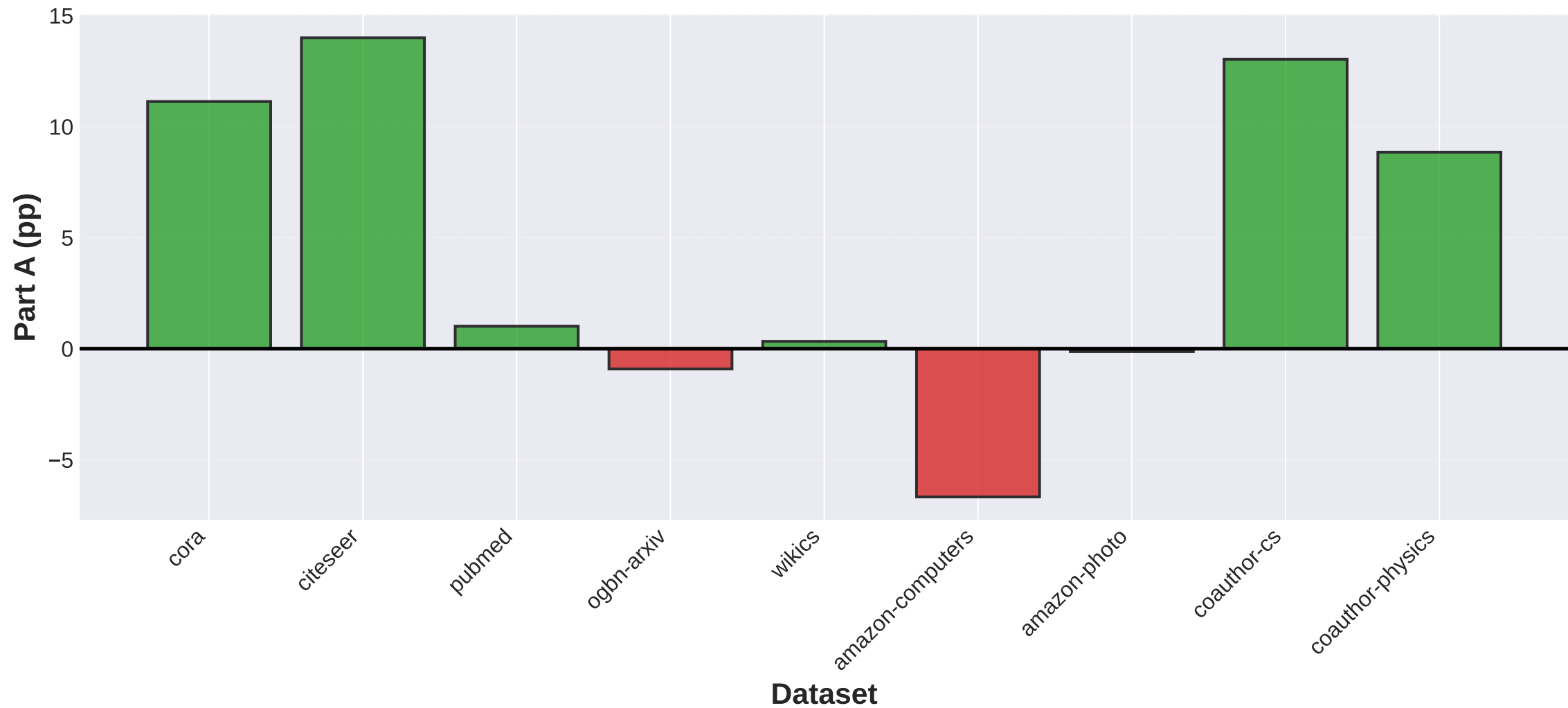
Basis Sensitivity Across Datasets (k=10, Random Splits)
