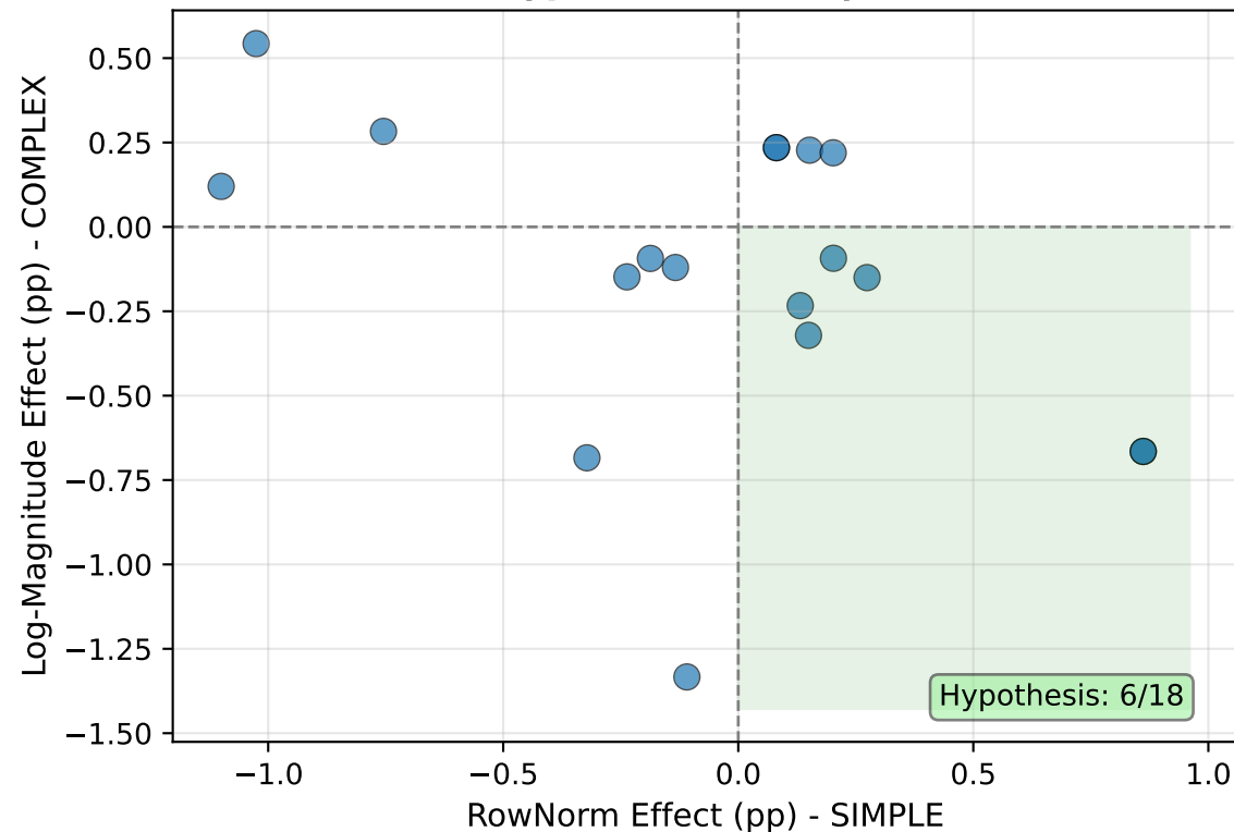
RowNorm vs Log-Magnitude Hypothesis: x > 0, y < 0
