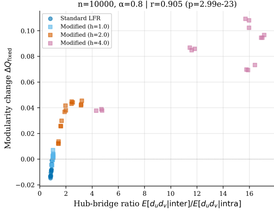
Fig. 3. Fixed-partition modularity change under DSpar as a function of induced hub-bridging on LFR graphs ( n = 10^4 , nominal \alpha = 0.8 , planted partitions). The controlled rewiring operator ( h : endpoint choice \propto d^h ) restores the coupling between hub-bridging, \delta , and \Delta Q_{\text{fixed}} .
