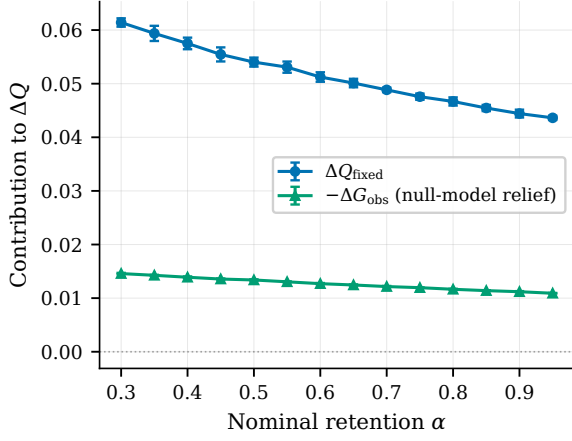
Fig. 1. Modularity decomposition under DSpar sparsification on cit-HepTh: \Delta Q_{\text{fixed}} alongside the null-model contribution -\Delta G_{\text{obs}} across sparsification levels; the remainder is \Delta F_{\text{obs}} (Table 3).
