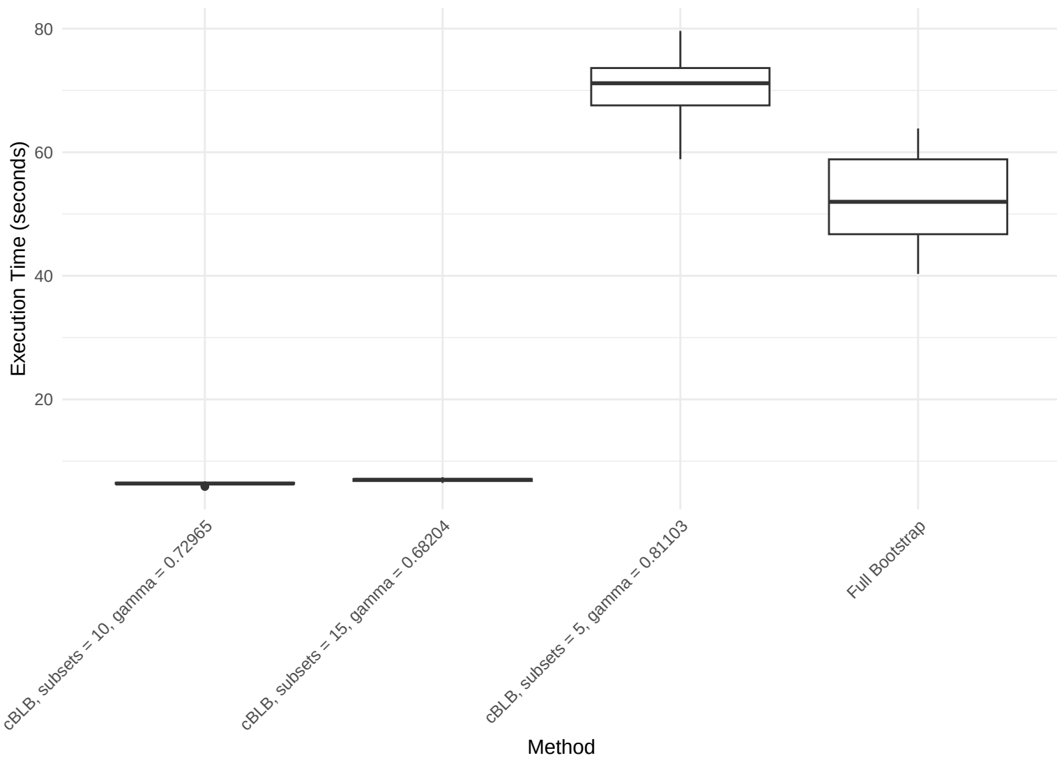
Timing Results by Method, Kernel Minimax Weights
