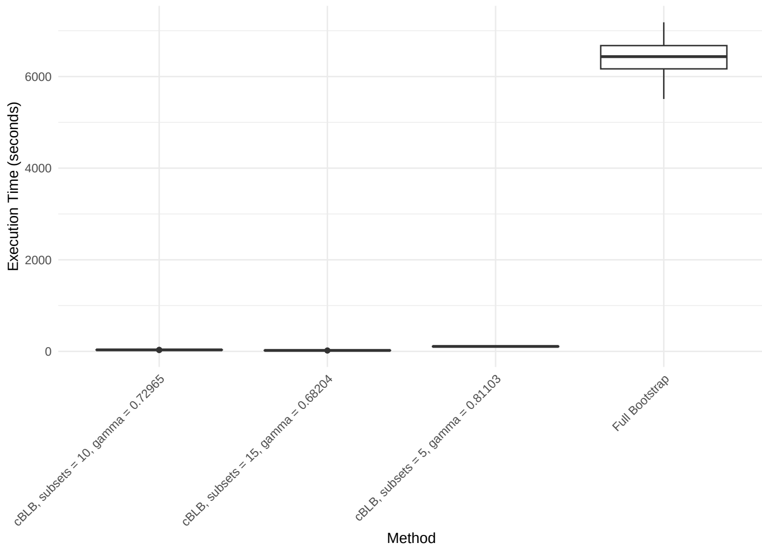
Timing Results by Method, Kernelized AOL
