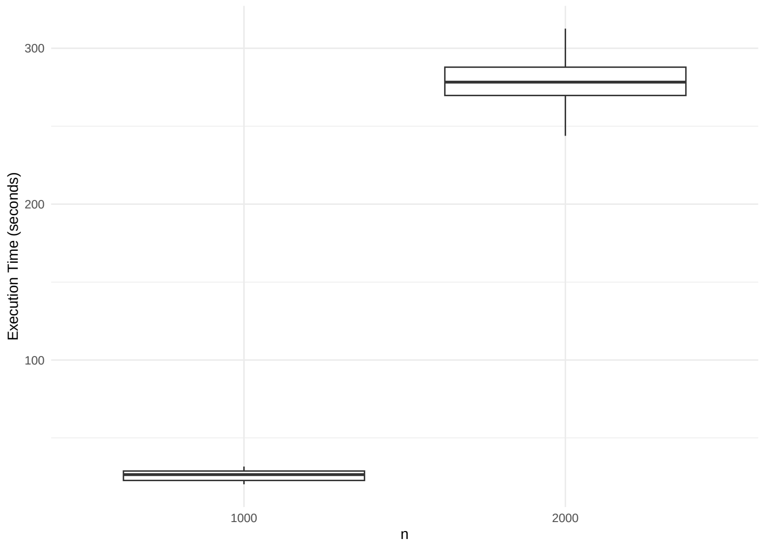
Full bootstrap, Kernelized AOL, by n size
