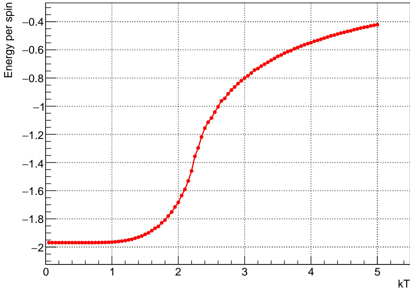
Energy vs Temperature ( h=0 )
