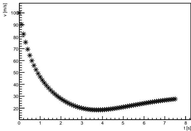
Projectile velocity vs t
