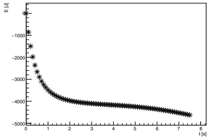
Projectile Etot-E0 vs t
