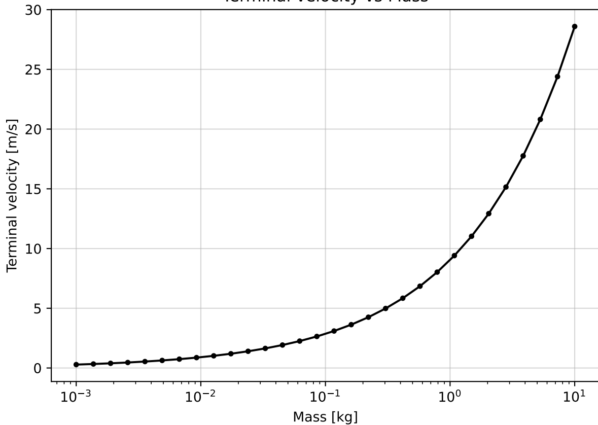
Terminal velocity vs Mass
