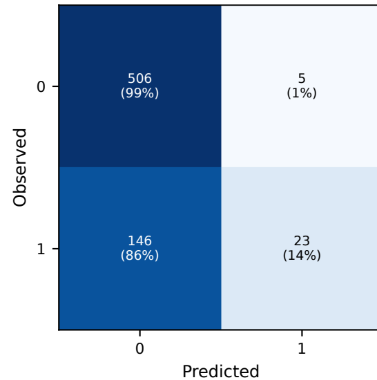
Logistic Regression
