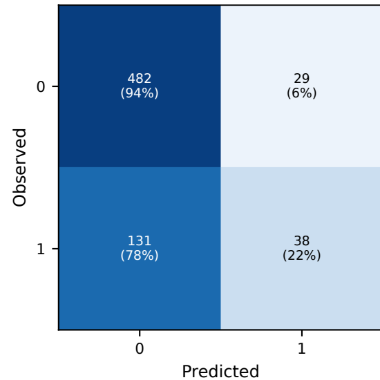
LightGBM
