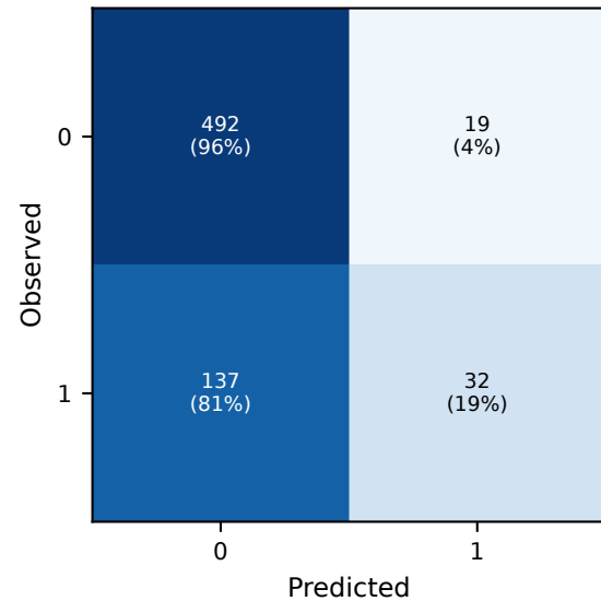
XGBoost
