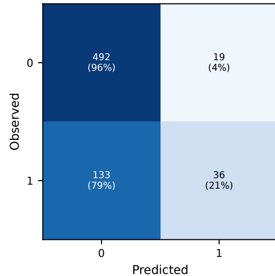
Random Forest
