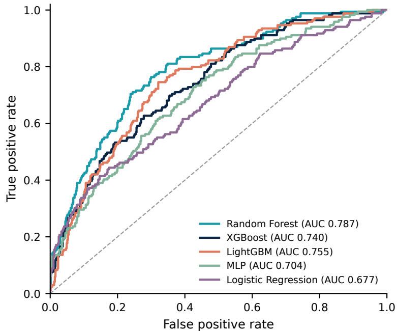
(a) ROC curves
