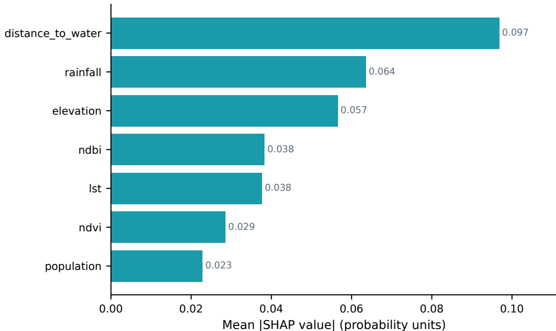
Global feature importance (mean |SHAP|)
