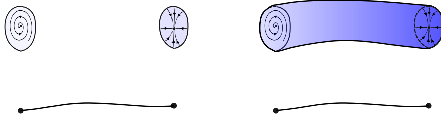
FIGURE 3. Continuation of asymptotically stable vector fields.
