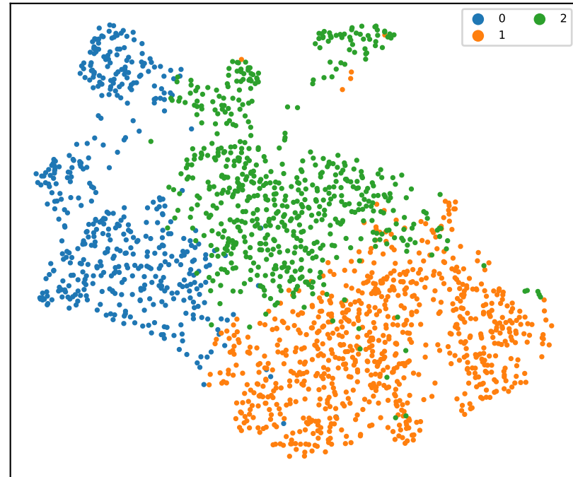
HDBSCAN clusters
