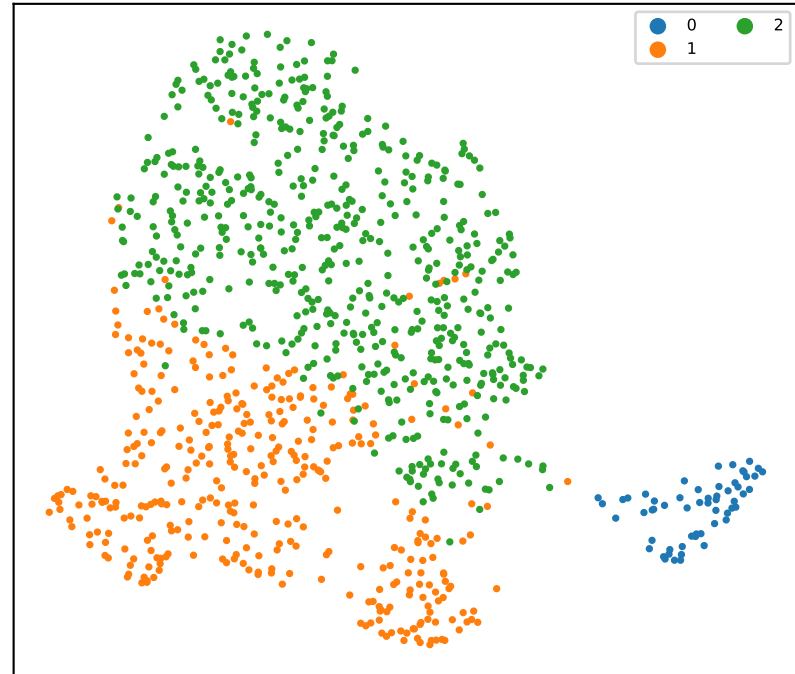
HDBSCAN clusters
