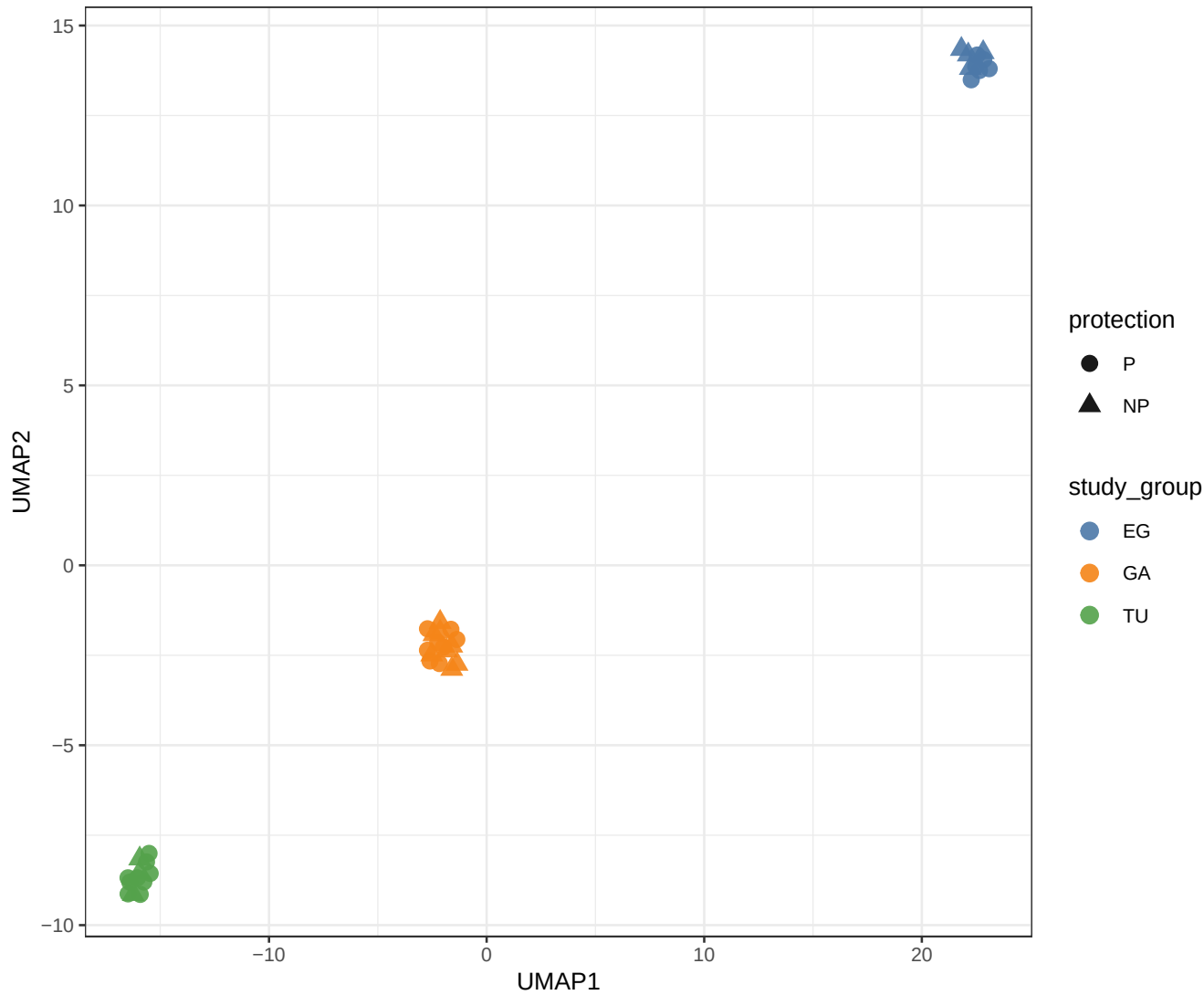
UMAP on selected or fallback immune–signature features
