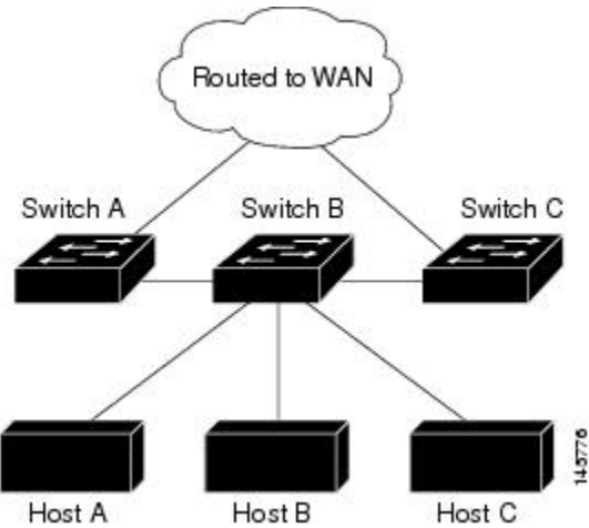
Figure 8: EIGRP Stub Router Configuration
