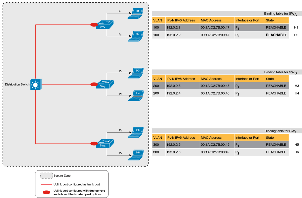
Figure 35: Secure Zone 2 - Efficient and Scalable Secure Zone When Binding Tables are Decentralized
