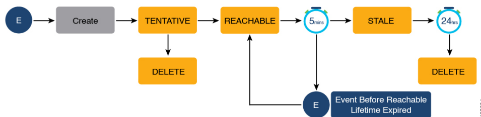
Figure 29: Lifecycle of an Entry
