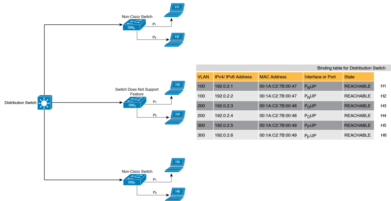
Figure 33: Centralised Binding Table
