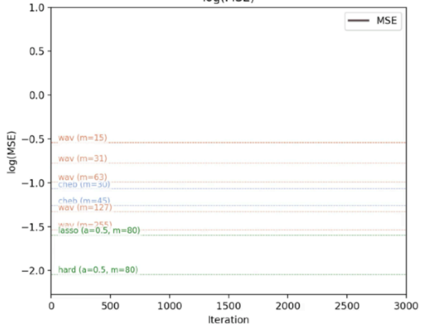
log(MSE)
