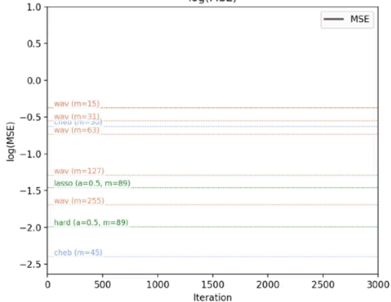
log(MSE)
