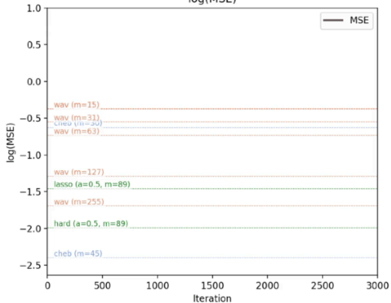
log(MSE)
