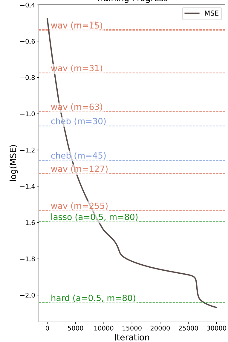
Training Progress
