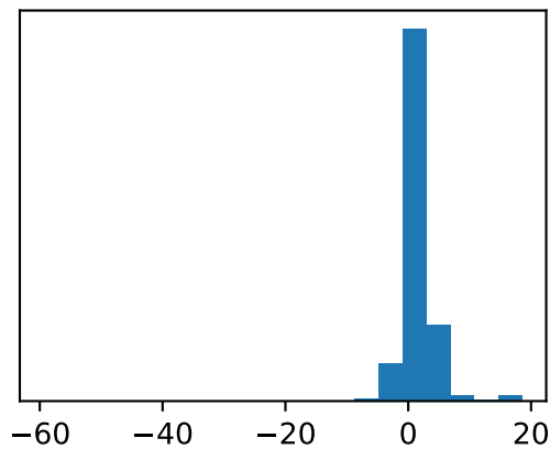
residuals
