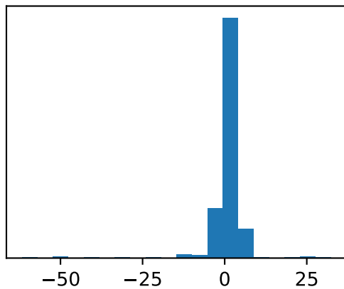
residuals
