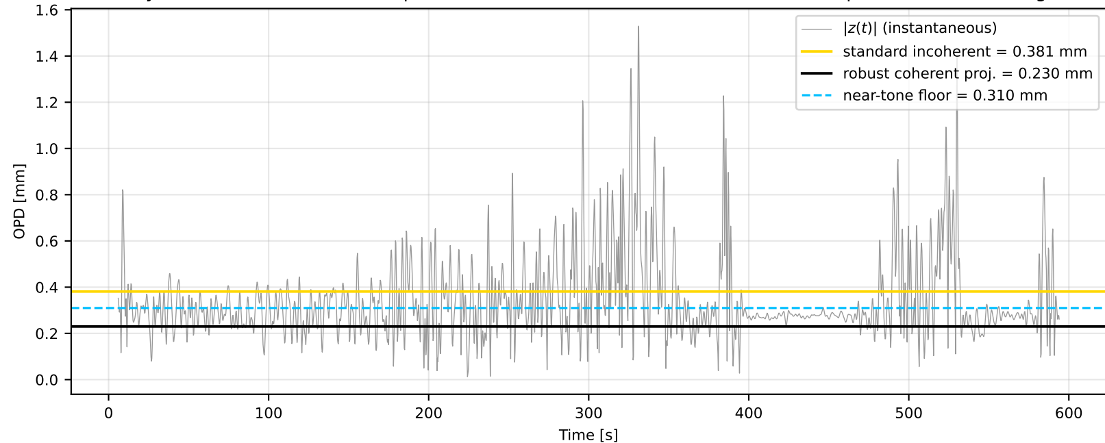
Rattly record (R2, NOSHIMS+torqued): the incoherent RMS sums in-band motion power as if it were signal
