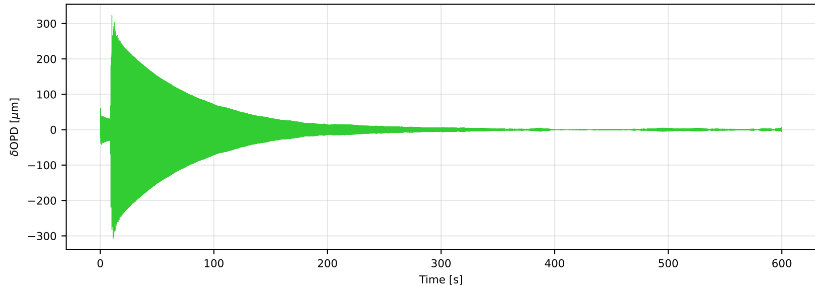
Test-mass motion from the low-frequency differential phase (band 0.5-45 Hz), RMS 46 \mu\text{m}
