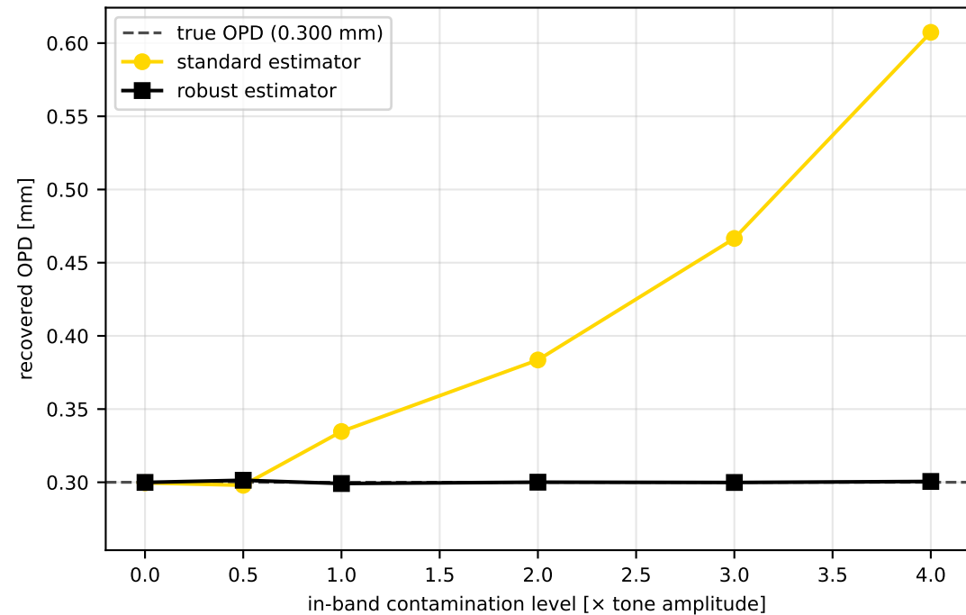
Bursty in-band contamination
