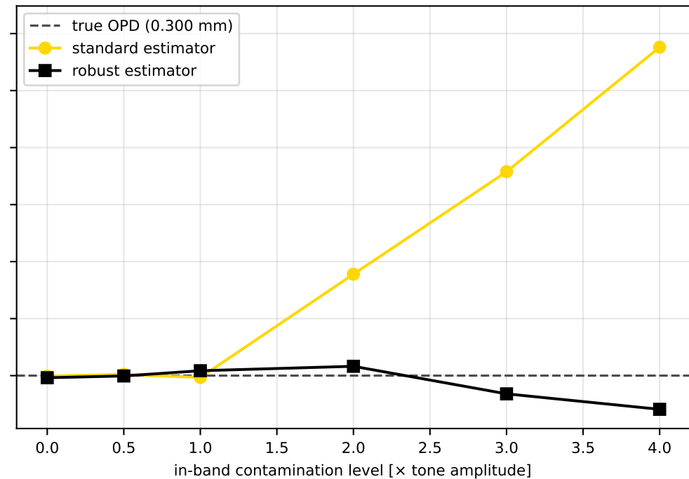
Steady in-band contamination
