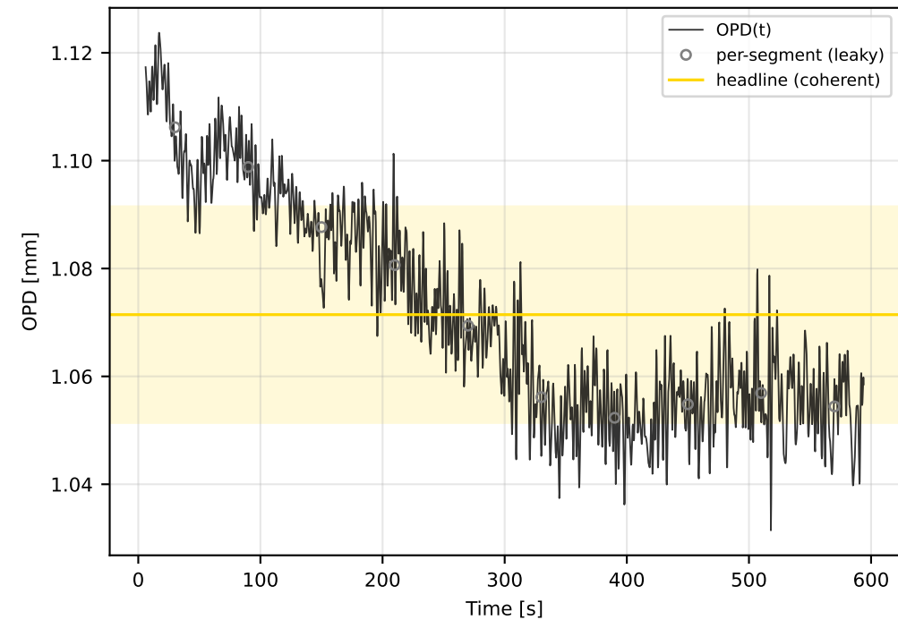
OPD = 1.0714 mm (drift \pm 0.0200 , noise \pm 0.41 \mu\text{m} )
