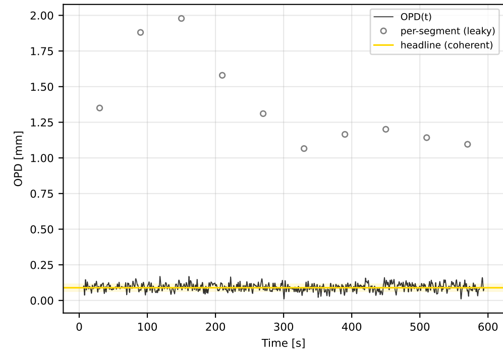
OPD = 0.0892 mm (drift \pm 0.0246 , noise \pm 1.42 \mu\text{m} ) coherence 1.00, leakage \times 1.8 , df 0.48 mHz
