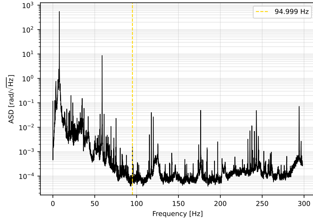
FM1Day09_VacuumReleasedOPD_SHIMMED_FLIGHTTORQUED_R1_20260629_140109 Differential phase (ch1-ch2)
