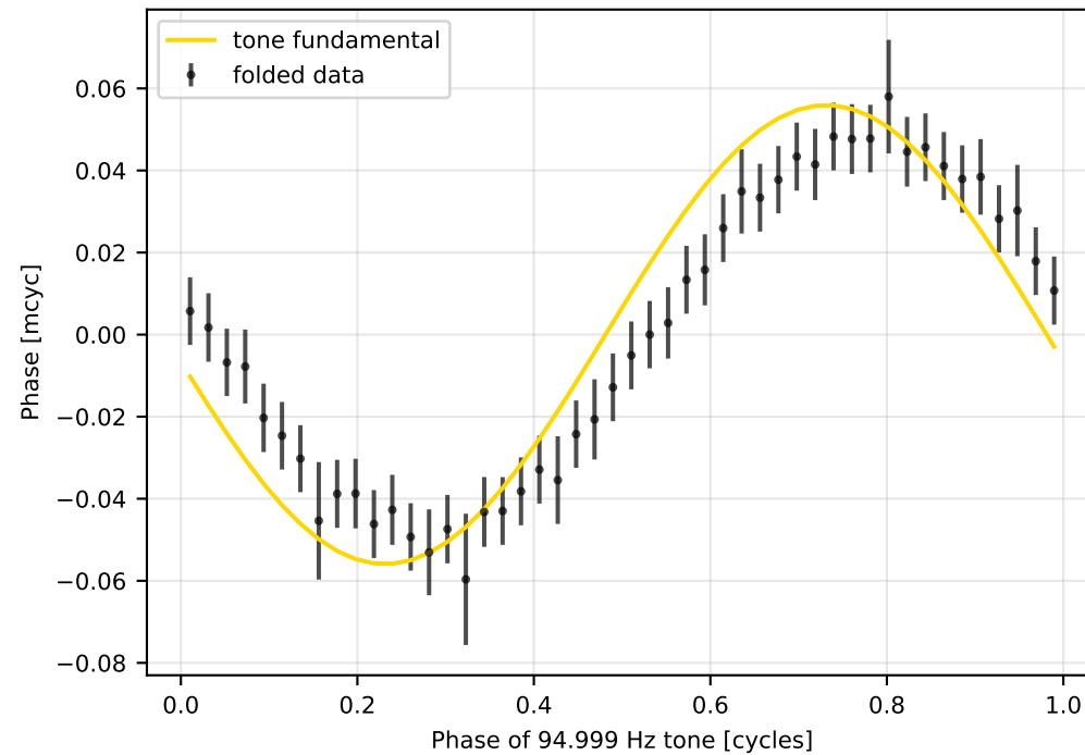
Folded tone: A = 5.593\text{e-}05 cyc (SNR 62.7)
