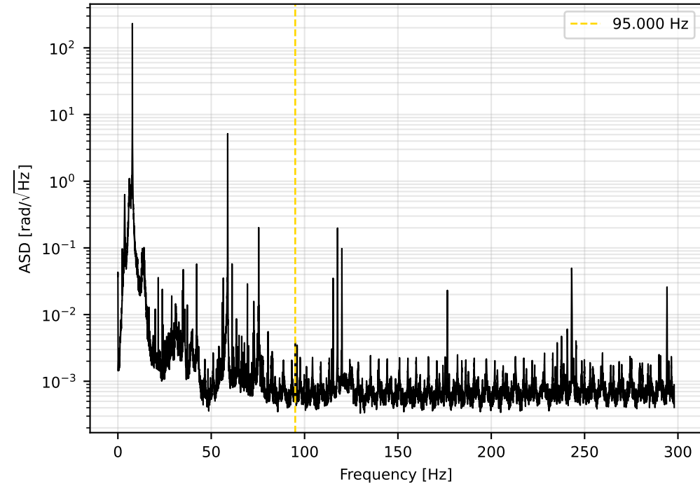
FM1Day09_VacuumReleasedOPD_SHIMMED_FLIGHTTORQUED_R2_20260629_140110 Differential phase (ch1-ch2)
