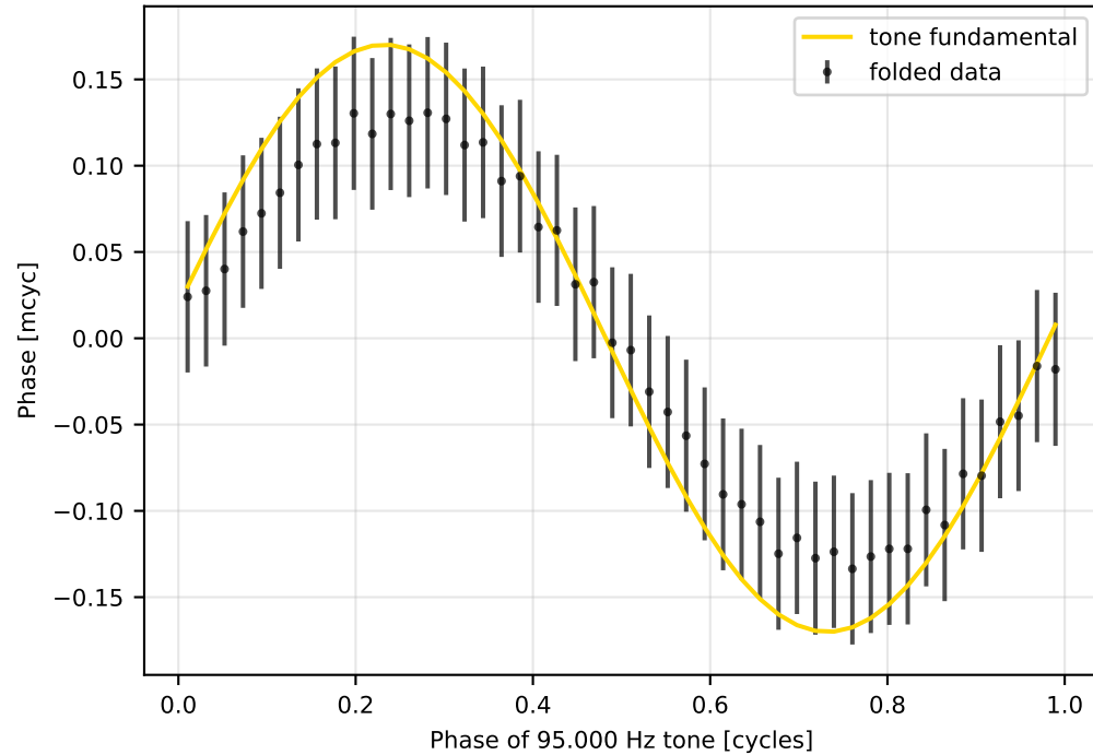
Folded tone: A = 1.701\text{e-}04 cyc (SNR 27.7)
