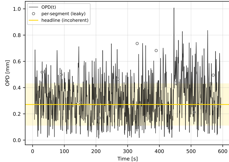
OPD = 0.2713 mm (drift \pm 0.1583 , noise \pm 9.79 \mu\text{m} ) coherence 0.09, leakage \times 1 , df -8.52 mHz
