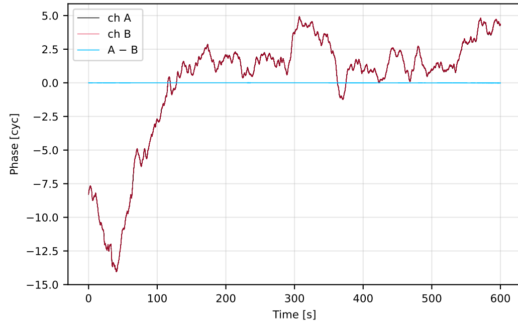
Per-channel wander cancels in the difference
