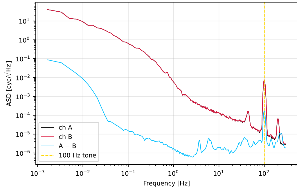
Tone is common-mode; residual OPD survives in A-B
