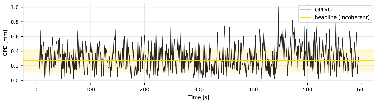
Case C (R2, released, vacuum): OPD=0.2713 mm, drift \pm 158 \mu\text{m} , noise \pm 9.79 \mu\text{m} , coh 0.09, leak \times 1.03
