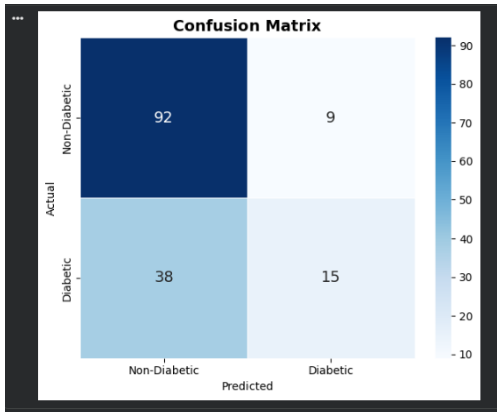
Figure 1: Confusion Matrix.
