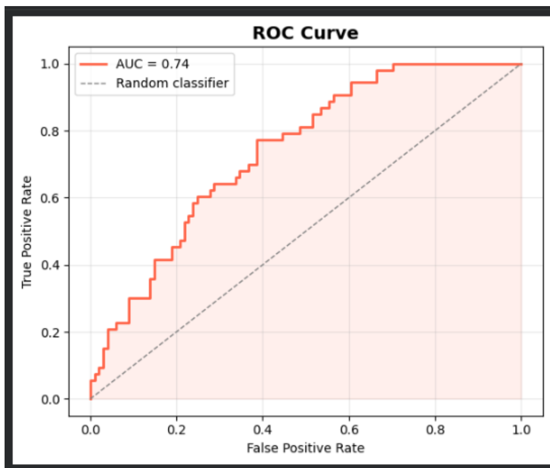
Figure 3: ROC curve.
