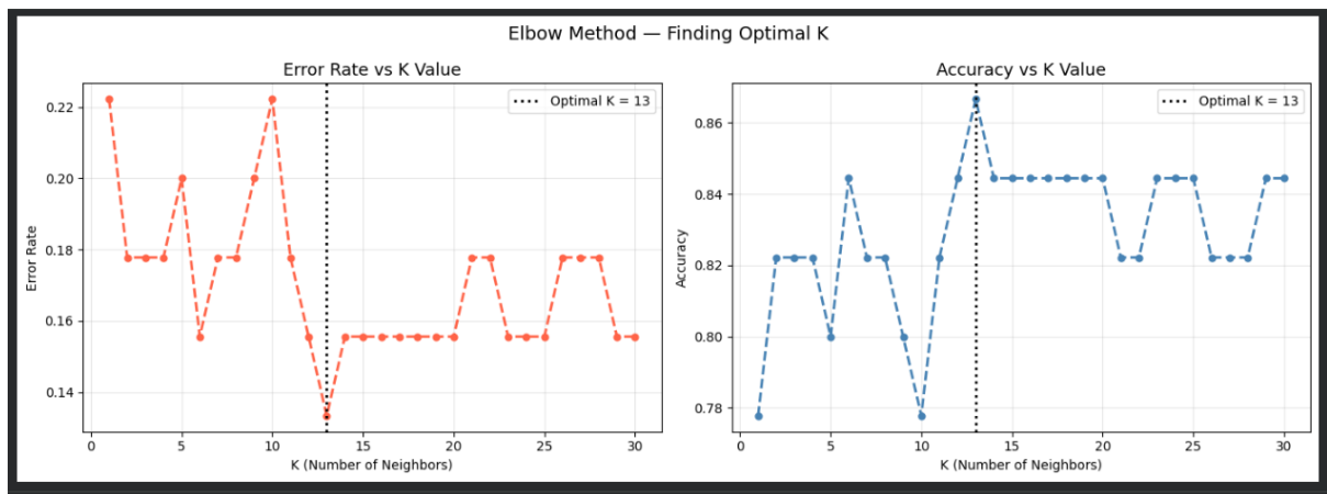
Figure 9: Elbow method plot.
