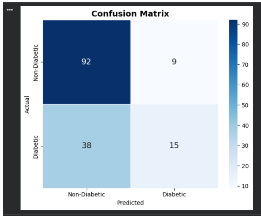
Figure 1: Confusion Matrix.
