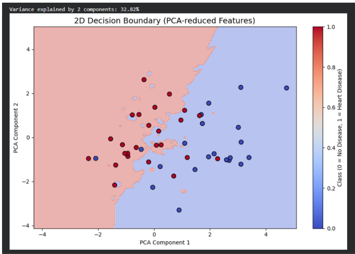
Figure 10: 2d decision boundary plot.
