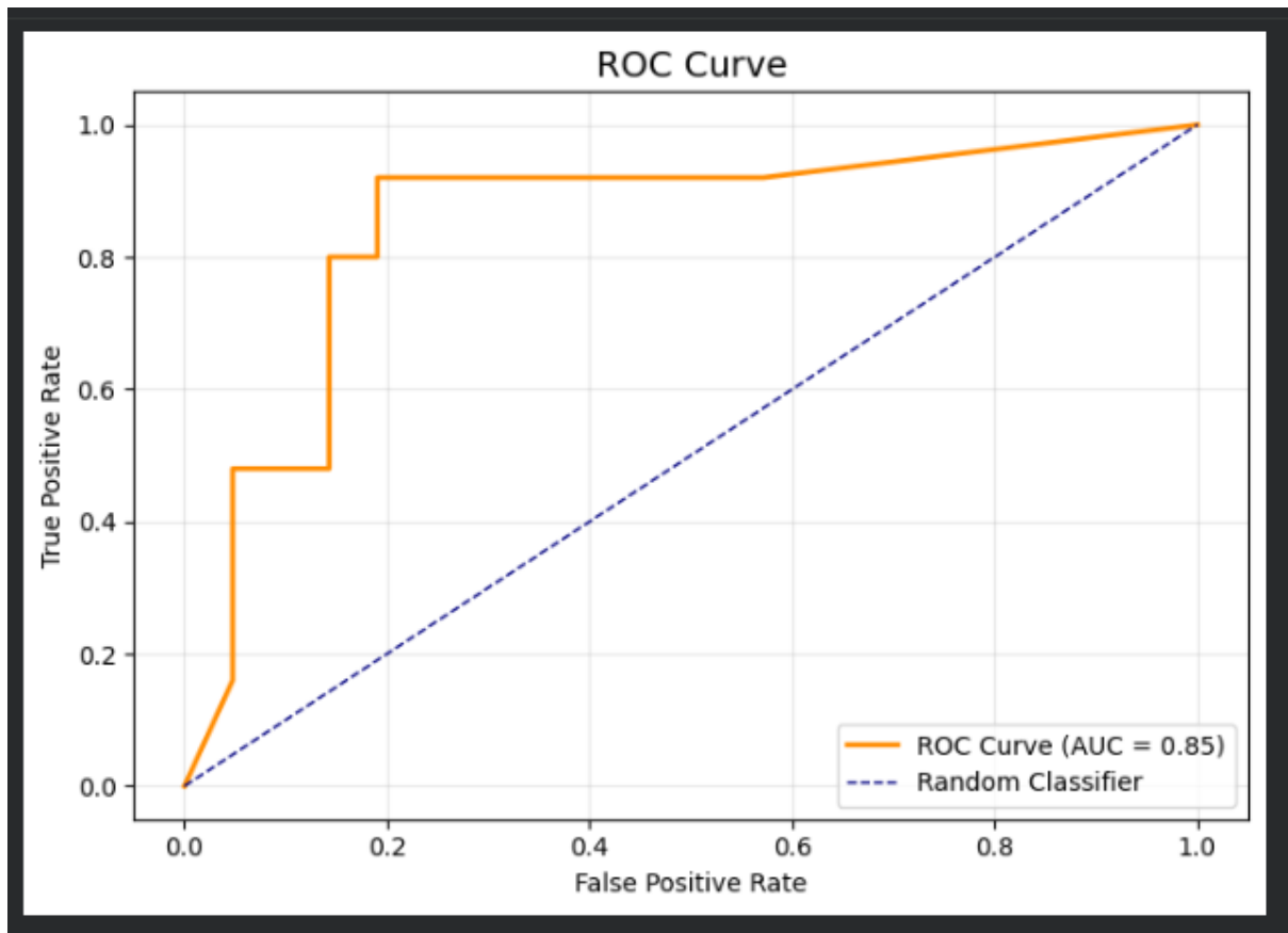
Figure 8: ROC Curve.
