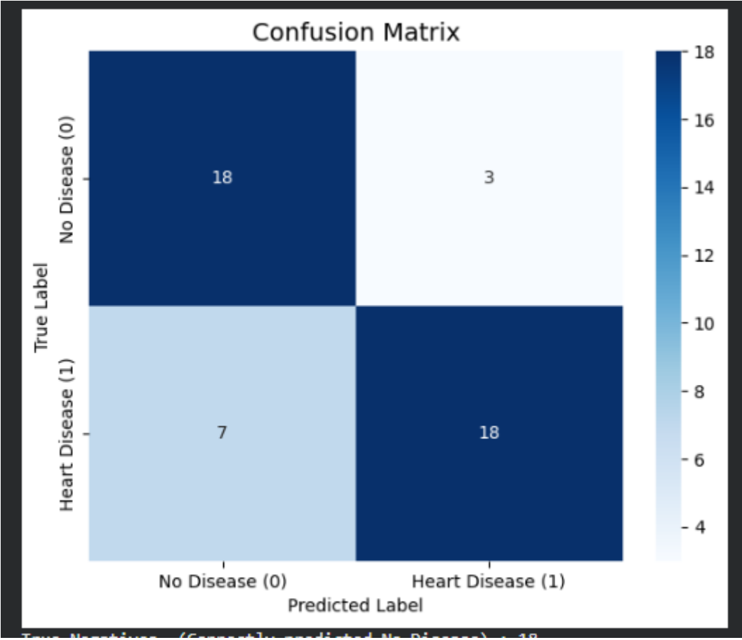
Figure 6: Confusion Matrix.
