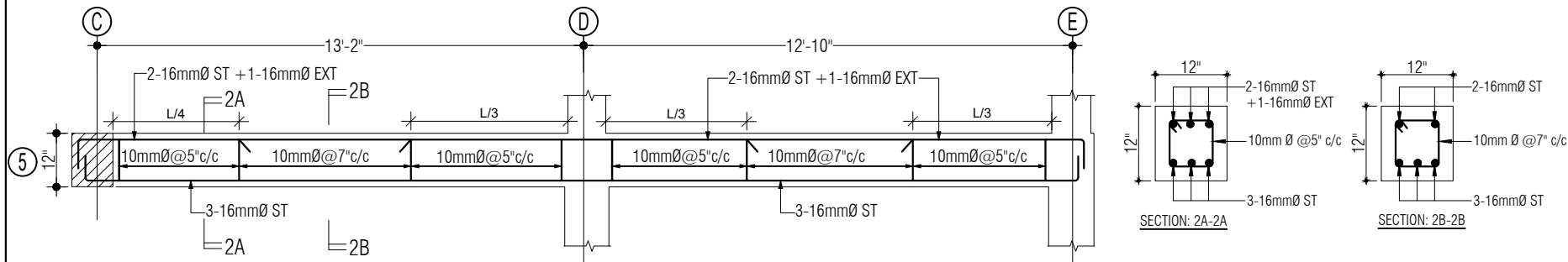
LONG SECTION OF GRADE BEAM GB-2 (12" x 12")
