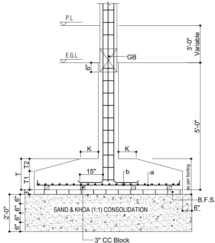
Typical footing section (A-A)
