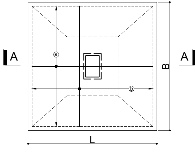
Plan of typical footing
