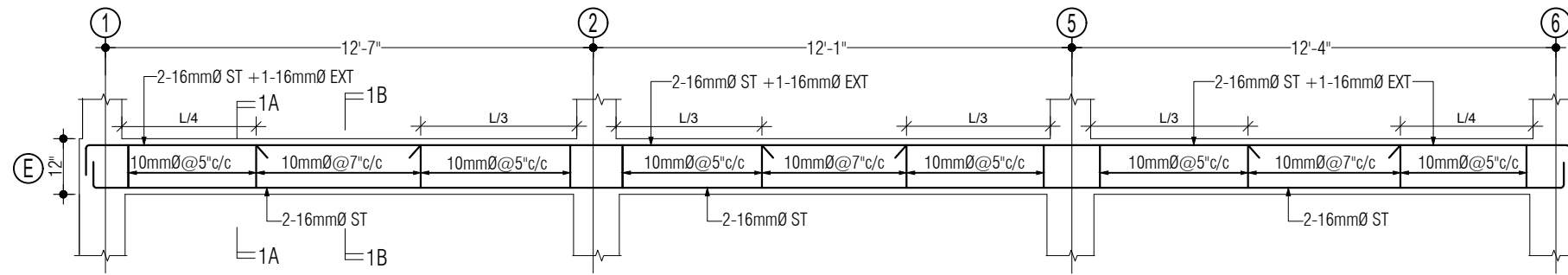
LONG SECTION OF GRADE BEAM GB-1 (12" x 12")
