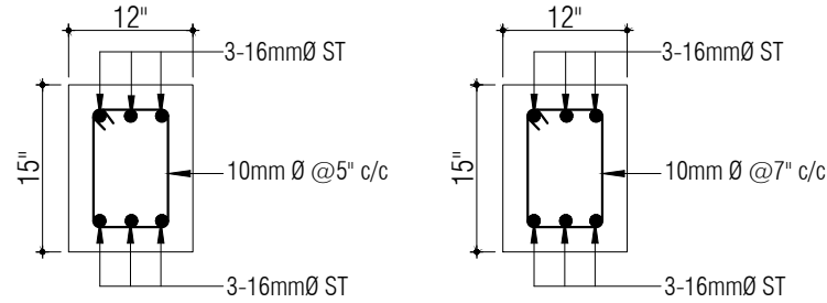
SECTION: 3A-3A
