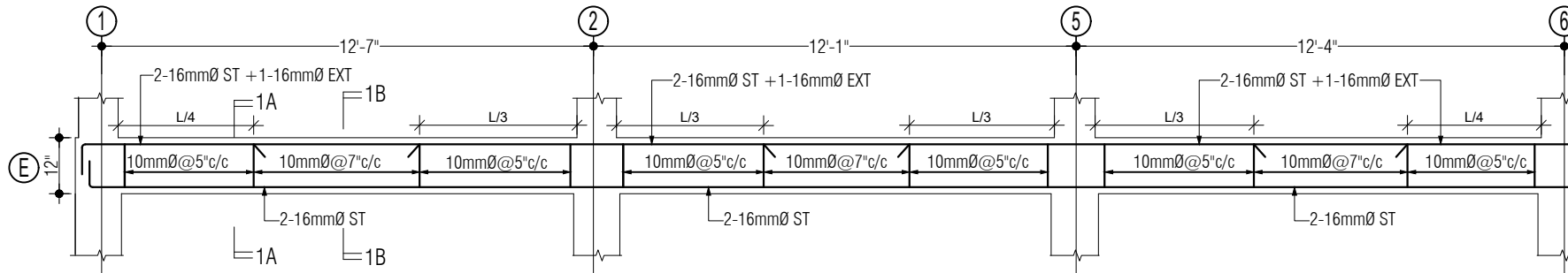
LONG SECTION OF GRADE BEAM GB-1 (12" x 12")
