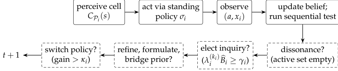
Figure 2: The period timeline. Solid steps occur every period: the agent perceives its current awareness cell, acts through its standing policy, observes the realized action profile and its own consequence, and updates its beliefs and sequential test (assumptions 3.3 and 3.4 and definition 5.1). Dashed steps are contingent: dissonance occurs only if the active set empties (definition 5.3); a dissonant agent elects inquiry only if \lambda_i^{(k_i)} \hat{B}_i \geq \gamma_i (proposition 7.4); a successful election refines awareness, and formulation with a bridge prior restores judgment (section 8); a policy switch occurs only when the horizon- T gain clears the hurdle \kappa_i (assumption 3.4).
