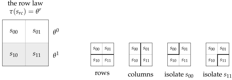
Figure 3: The four-state laboratory. Left: states s_{rc} with the row law \tau(s_{rc}) = \theta^r —the row coordinate is causally relevant, the column coordinate is not ( example 1 ). Right: once the discovery record labels s_{00} and s_{11} , exactly four minimal repairs separate them (thick boundaries): the row partition, the column partition, and the two partitions isolating one labeled state ( section 6 ).
