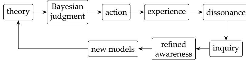
Figure 1: The organizing chain. A theory supports Bayesian judgment and action; experience can defeat every expressible theory, producing causal dissonance; costly inquiry may refine awareness; formulation on the refined language yields new models and a new theory, and Bayesian judgment resumes.
