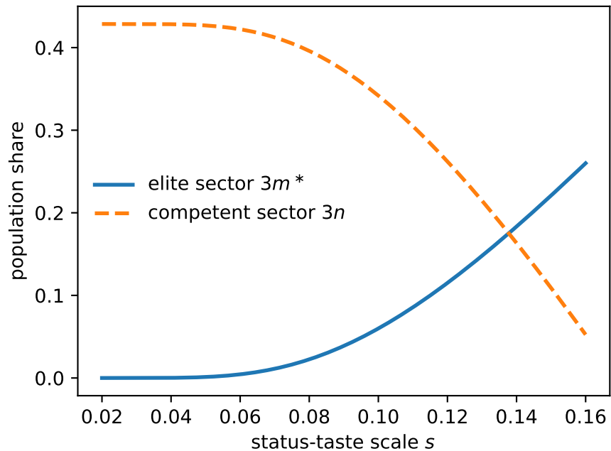
(a) Sorting
