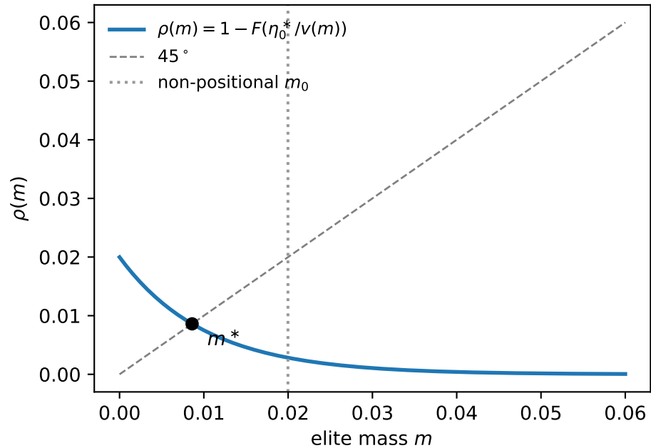
(a) Unique positional equilibrium
