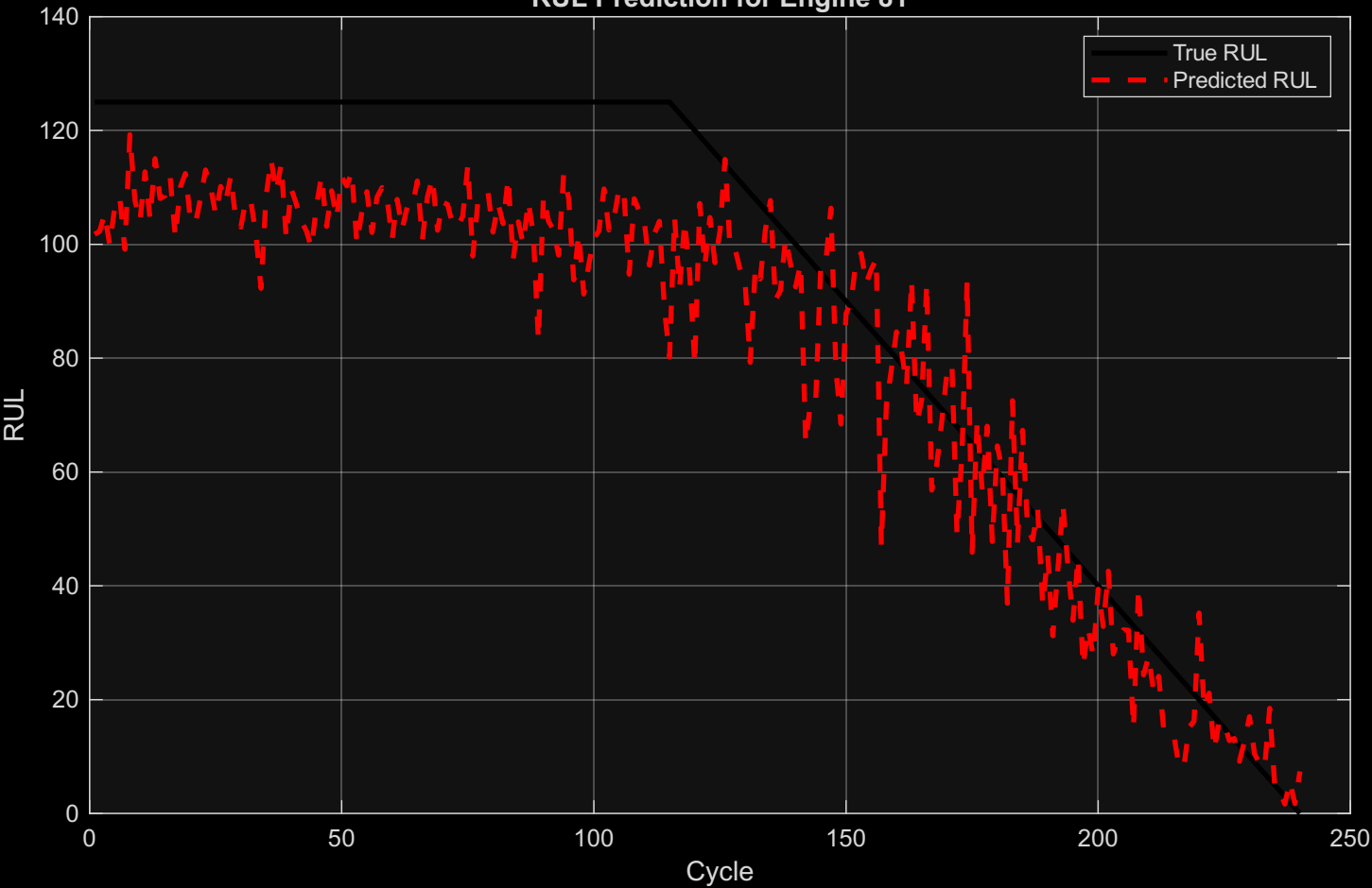
RUL Prediction for Engine 81
