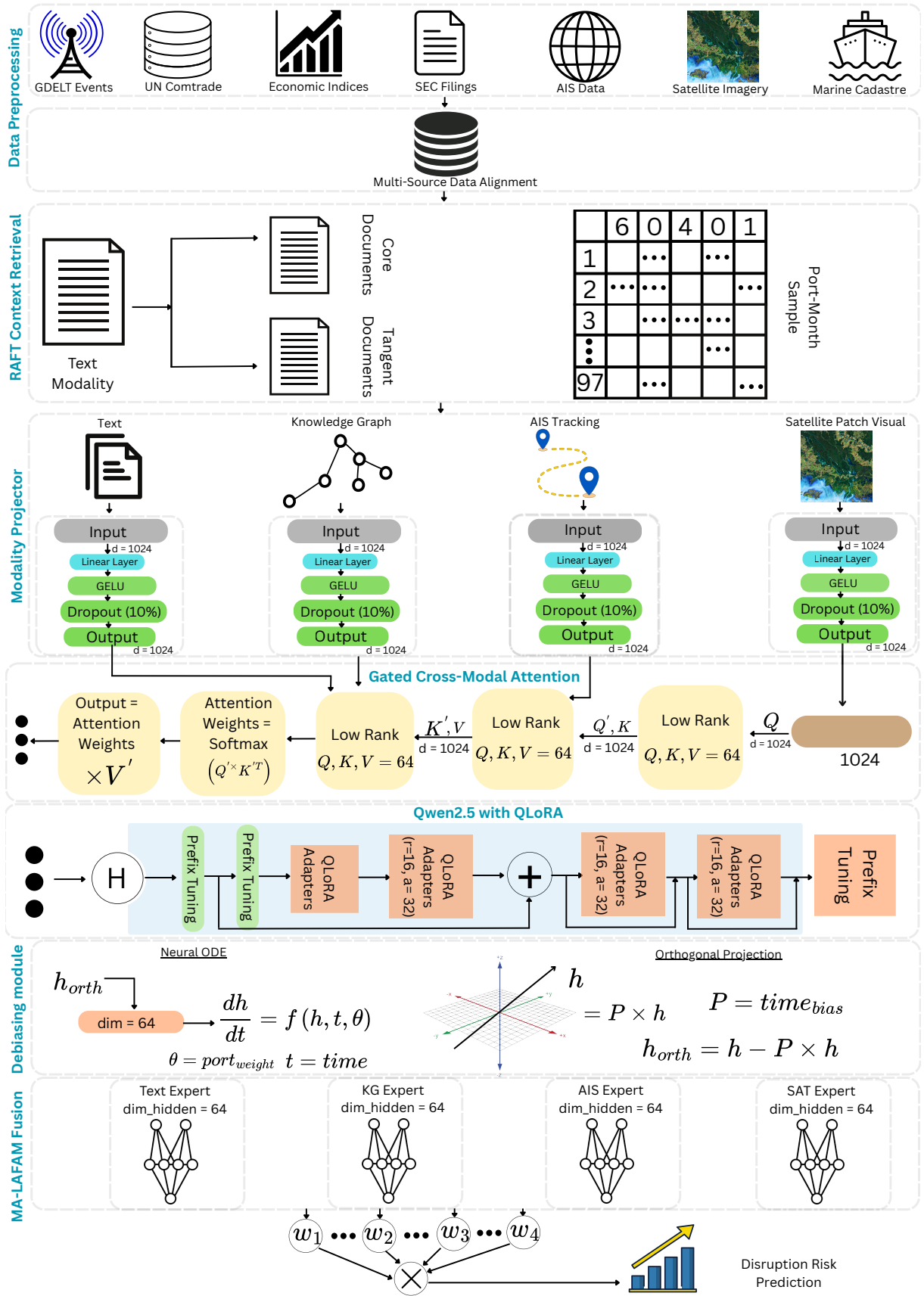
Figure 2: CauSAIL workflow for port-month maritime supply chain disruption detection.
