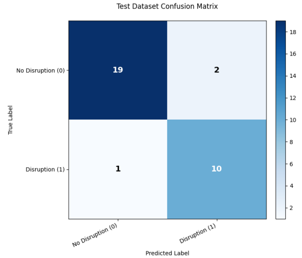
Figure 1: Confusion matrix of CauSAIL.
