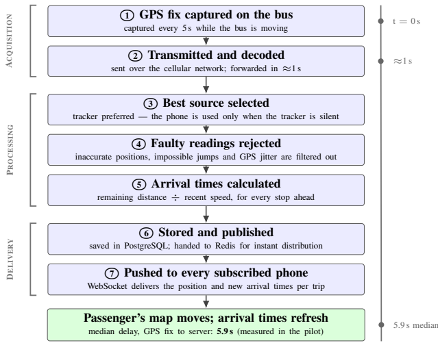
Fig. 2. Real-time data flow: the life of one position report, from the GPS fix on the bus to the passenger's screen, grouped into acquisition, processing, and delivery phases. Steps 3–5 are detailed in Sections IV-A–IV-C.
