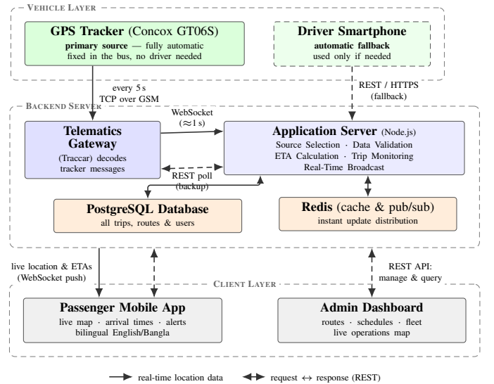
Fig. 1. UniBus Live system architecture. The fixed GPS tracker is the primary position source and operates with no driver involvement; the driver’s smartphone serves only as an automatic fallback. All backend components run on a single low-cost cloud server.
