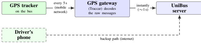
Fig. 2. How position reports travel from the bus to the UniBus server.
