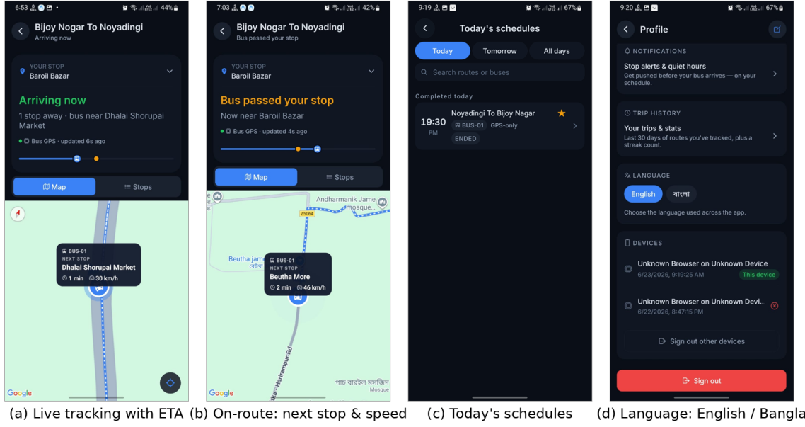
Fig. 6. The bilingual passenger application. (a) live tracking of a moving bus with the next-stop ETA; (b) on-route status showing the next stop and current speed; (c) today's schedules; (d) the in-app English/Bangla language toggle. Place names render in both scripts.
