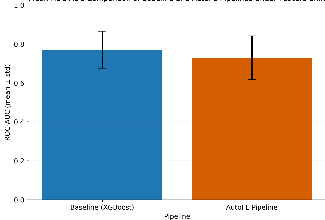
Mean ROC-AUC Comparison of Baseline and AutoFE Pipelines Under Feature Shift
