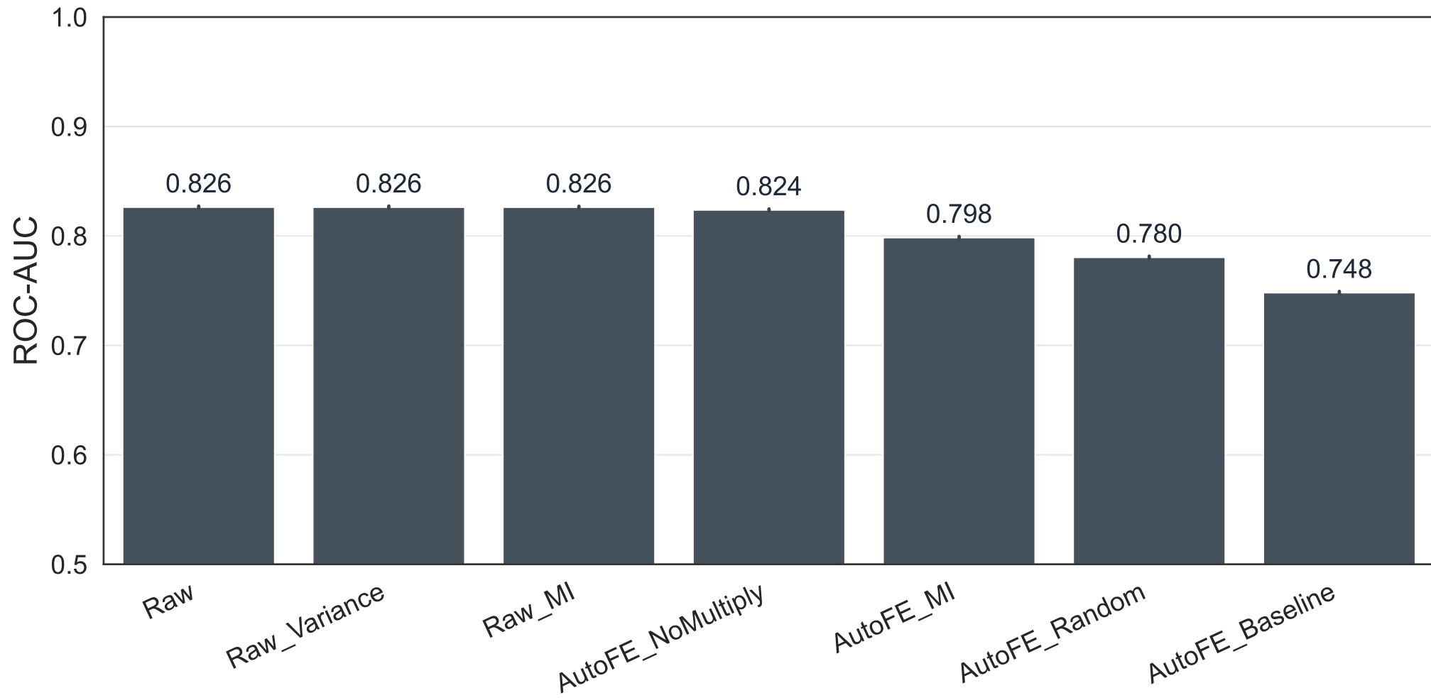
Figure 3: Overall Pipeline Ranking (Mean ROC-AUC)
