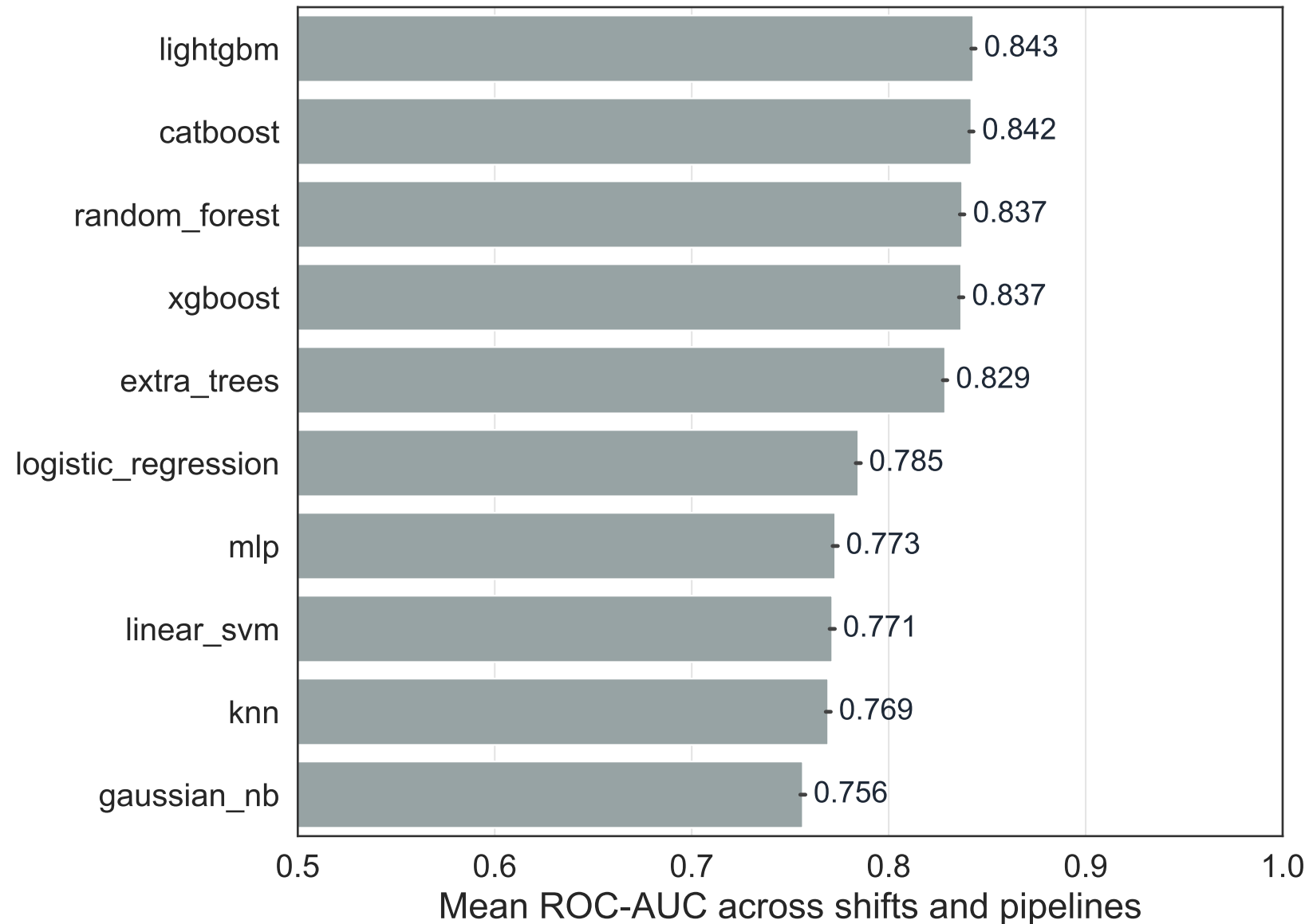
Figure 4: Classifier Robustness Ranking
