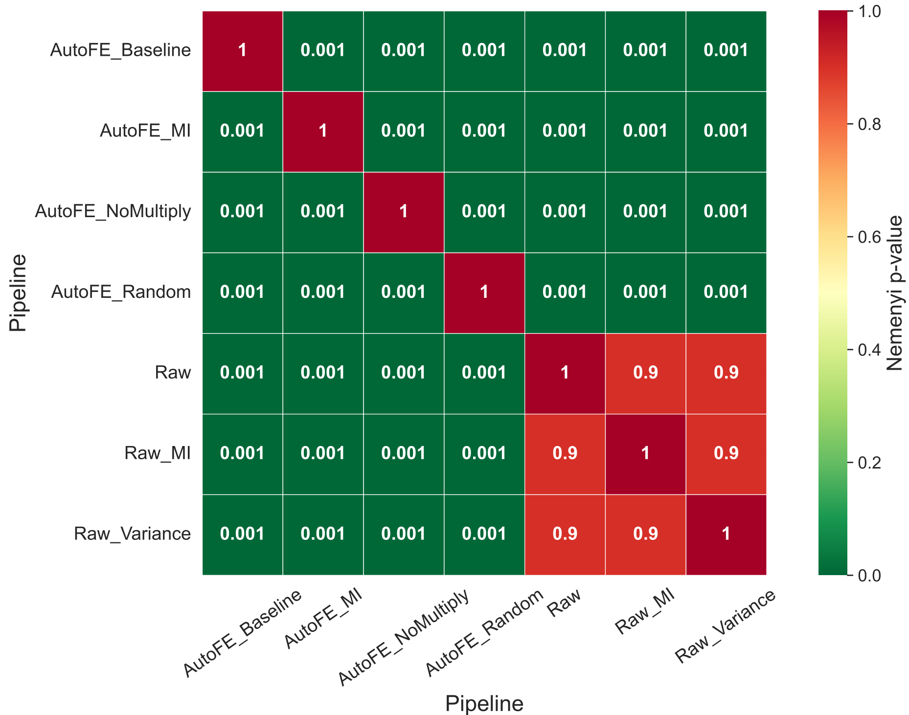
Figure 8: Nemenyi Post-hoc P-value Heatmap
